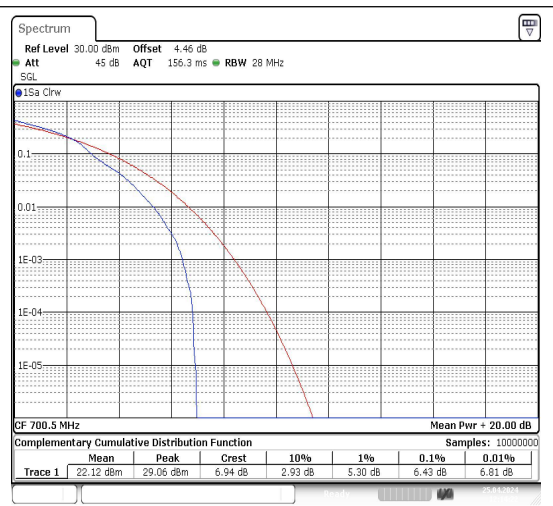
Band12-3MHz-16QAM-23025-1RB#0-PASS
