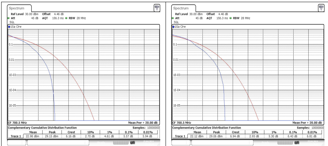
Band12-3MHz-QPSK-23025-1RB#0-PASS
