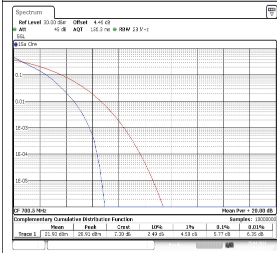
Band12-3MHz-QPSK-23025-1RB#0-PASS
