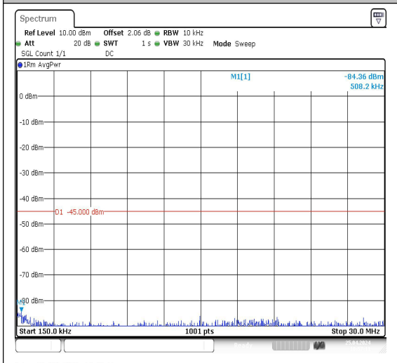
Band7_20MHz_16QAM_20850_1RB#0_0.15~30_0.15~30
