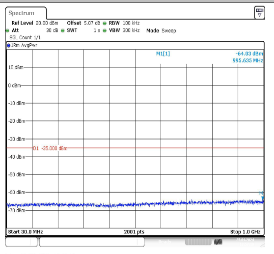
Band7_20MHz_16QAM_20850_1RB#0_30~1000_30~1000
