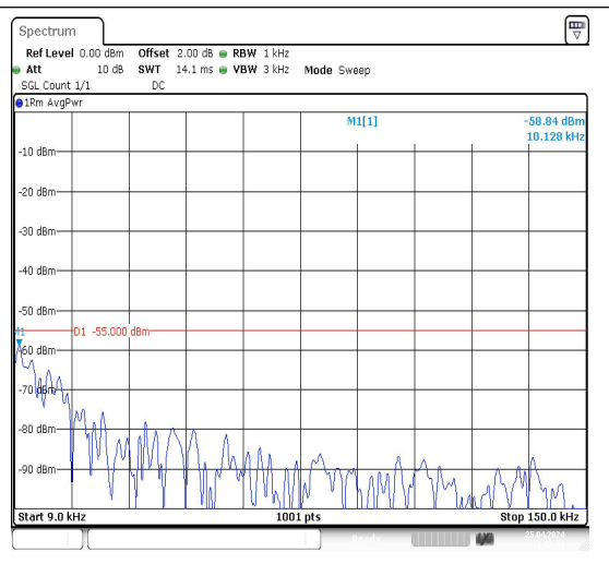
Band7_20MHz_16QAM_20850_1RB#0_0.009~0.15_5_0.009~0.15
