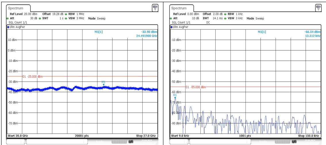
Band7_5MHz_QPSK_21425_1RB#0_20000~27000_00_20000~27000 Band7_5MHz_16QAM_21425_1RB#0_0.009~0.15_0.009~0.15
