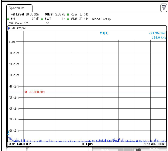
Band7_5MHz_QPSK_21100_1RB#0_20000~27000_20000~27000
