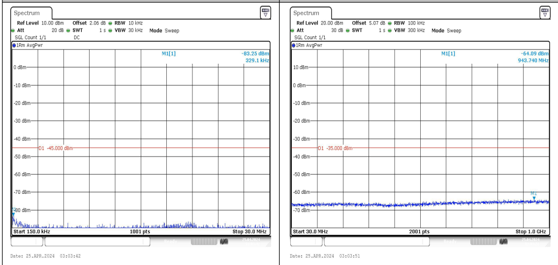
Band7_5MHz_16QAM_21425_1RB#0_0.15~30_0.15~30 Band7_5MHz_16QAM_21425_1RB#0_30~1000_30~1000
