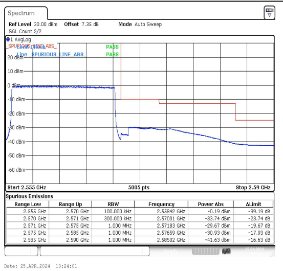
Band7_15MHz_16QAM_21375_75RB#0
