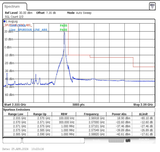
Band7_15MHz_16QAM_21375_1RB#74
