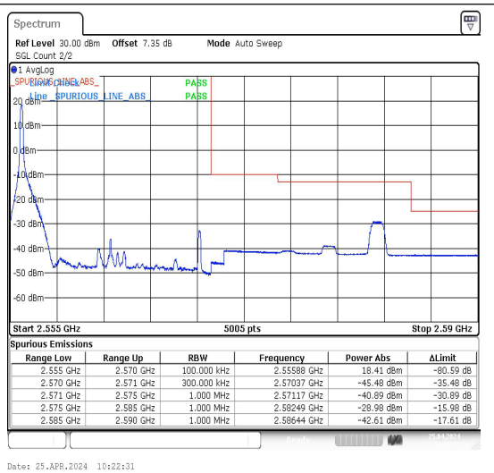
Band7_15MHz_16QAM_21375_1RB#0
