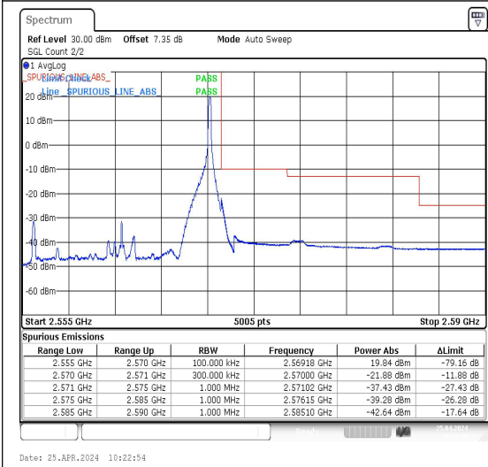
Band7_15MHz_QPSK_21375_1RB#74
