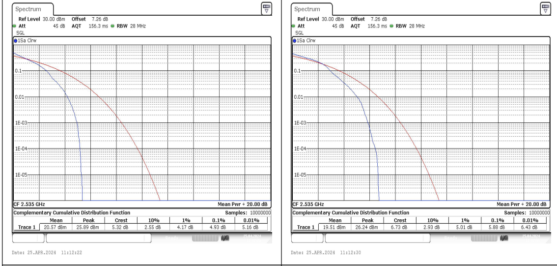
Band7-20MHz-QPSK-21100-1RB#0-PASS Band7-20MHz-16QAM-21100-1RB#0-PASS
