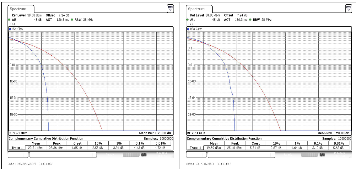
Band7-20MHz-QPSK-20850-1RB#0-PASS Band7-20MHz-16QAM-20850-1RB#0-PASS
