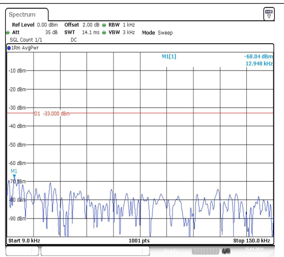
Band5_10MHz_16QAM_20600_1RB#0_0.009~0.15_0.009~0.15
