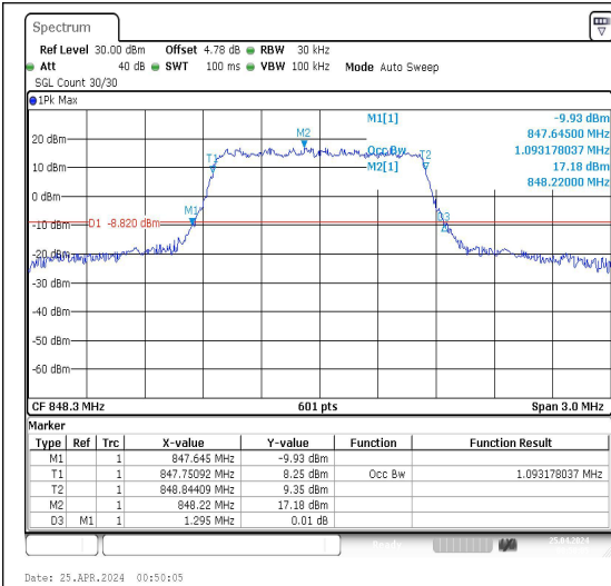
Band5-1.4MHz-QPSK-20643-6RB#0-PASS
