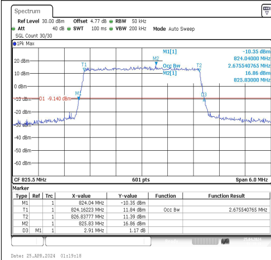
Band5-3MHz-QPSK-20415-15RB#0-PASS
