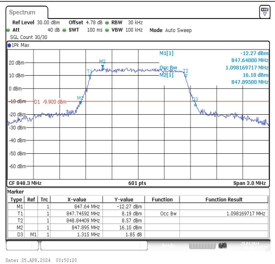
Band5-1.4MHz-16QAM-20643-6RB#0-PASS
