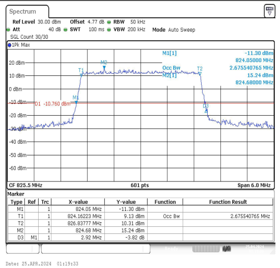
Band5-3MHz-16QAM-20415-15RB#0-PASS
