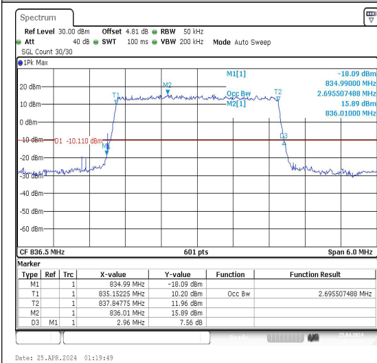
Band5-3MHz-QPSK-20525-15RB#0-PASS
