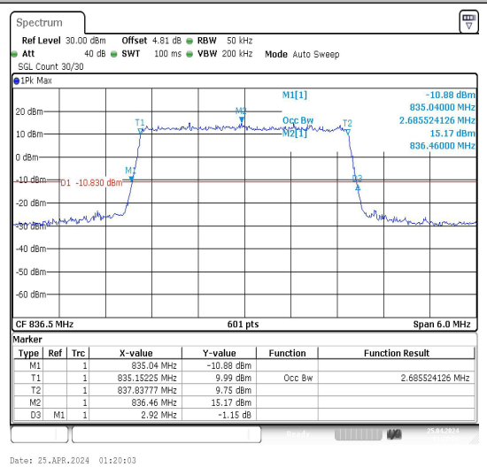
Band5-3MHz-16QAM-20525-15RB#0-PASS
