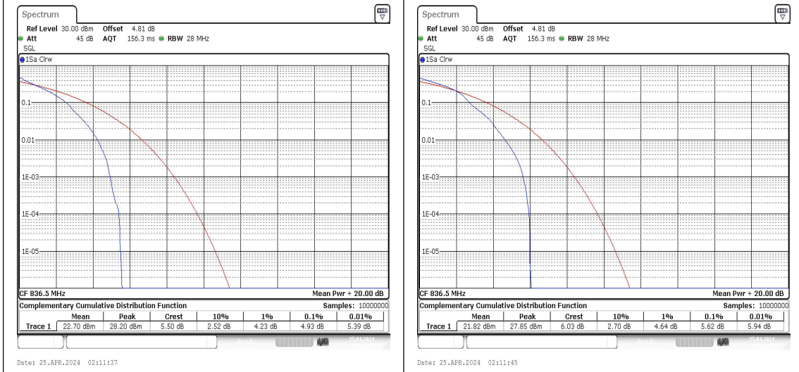
Band5-5MHz-QPSK-20525-1RB#0-PASS Band5-5MHz-16QAM-20525-1RB#0-PASS
