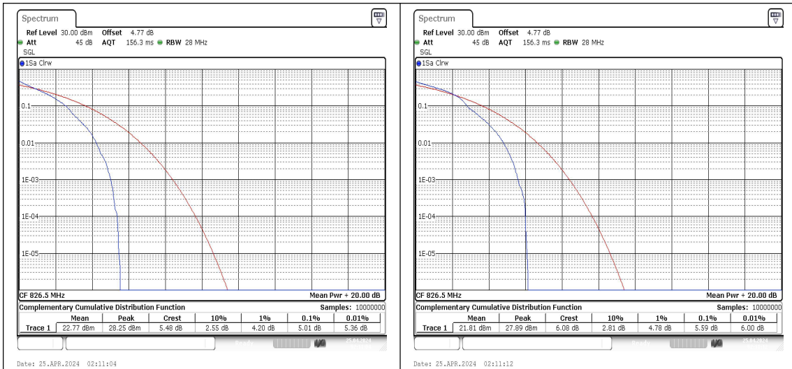
Band5-5MHz-QPSK-20425-1RB#0-PASS Band5-5MHz-16QAM-20425-1RB#0-PASS
