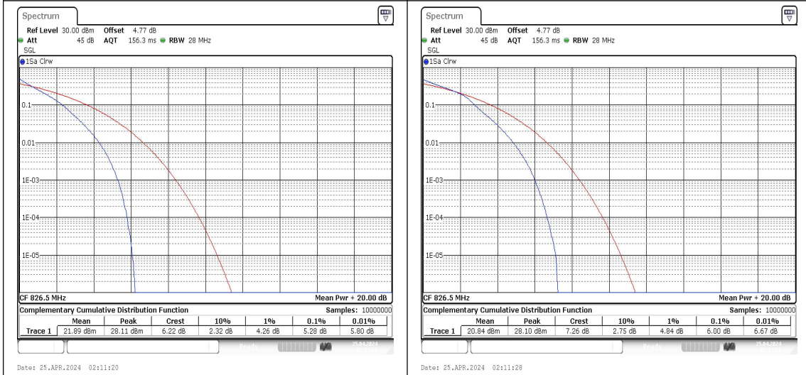
Band5-5MHz-QPSK-20425-25RB#0-PASS Band5-5MHz-16QAM-20425-25RB#0-PASS
