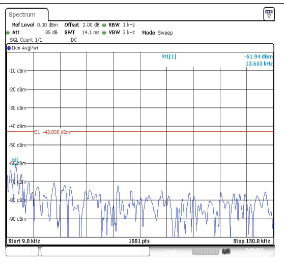
Band4_20MHz_16QAM_20050_1RB#0_0.009~0.15_0.009~0.15
