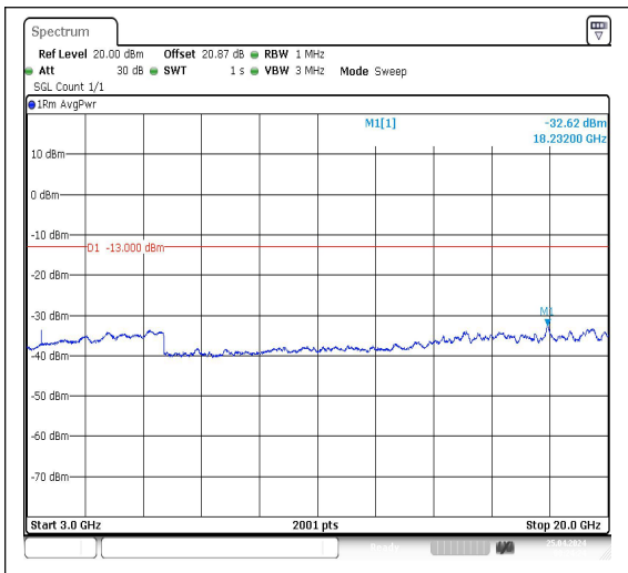
Band4_20MHz_QPSK_20050_1RB#0_3000~2000_3000~20000
