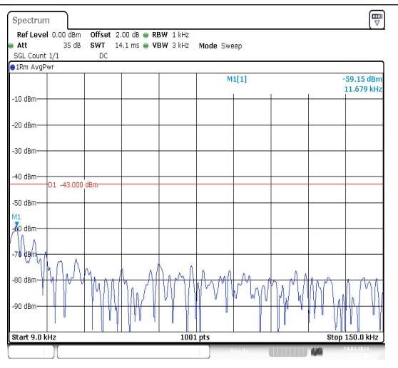
Band4_10MHz_16QAM_20350_1RB#0_0.009~0.15
