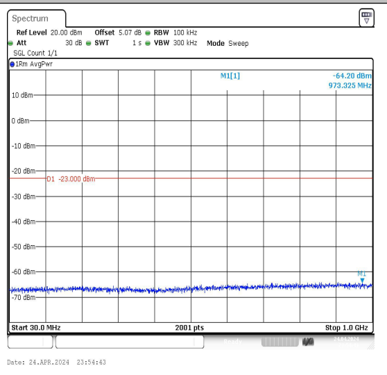
Band4_15MHz_16QAM_20025_1RB#0_30~1000_30~1000
