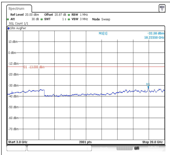
Band4_10MHz_QPSK_20350_1RB#0_3000~20000
