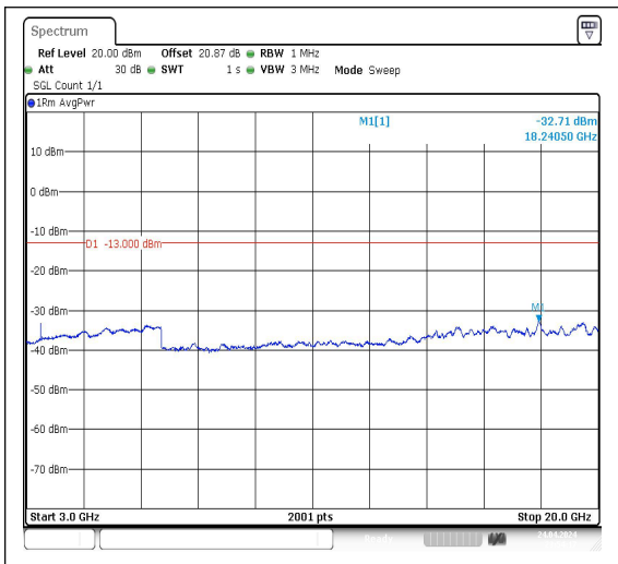
Band4_15MHz_QPSK_20025_1RB#0_3000~20000_00_3000~20000
