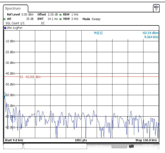
Band4_15MHz_16QAM_20025_1RB#0_0.009~0.15_5_0.009~0.15
