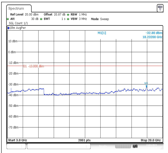
Band4_10MHz_QPSK_20000_1RB#0_3000~20000_00_3000~20000
