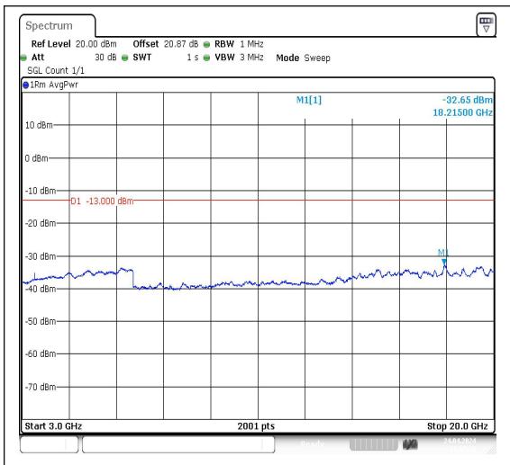
Band4_1.4MHz_QPSK_20175_1RB#0_3000~20000_00_3000~20000
