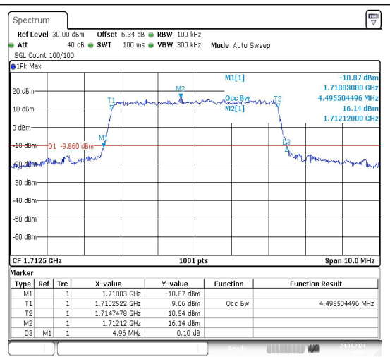
Band4-5MHz-16QAM-19975-25RB#0-PASS
