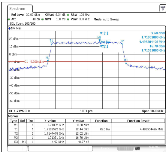
Band4-5MHz-QPSK-19975-25RB#0-PASS
