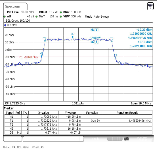
Band4-5MHz-16QAM-20175-25RB#0-PASS
