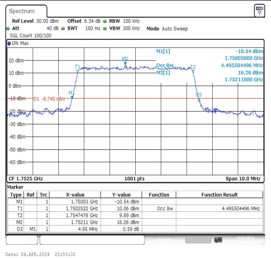
Band4-5MHz-16QAM-20375-25RB#0-PASS
