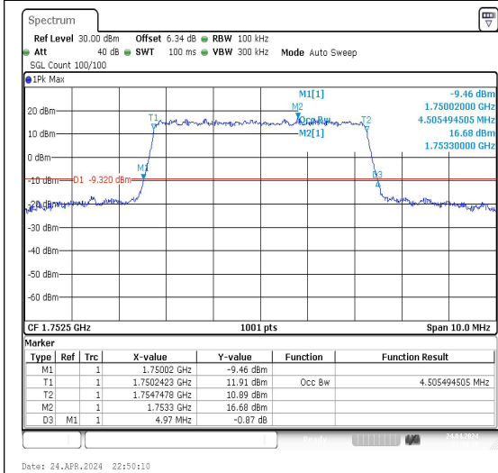
Band4-5MHz-QPSK-20375-25RB#0-PASS
