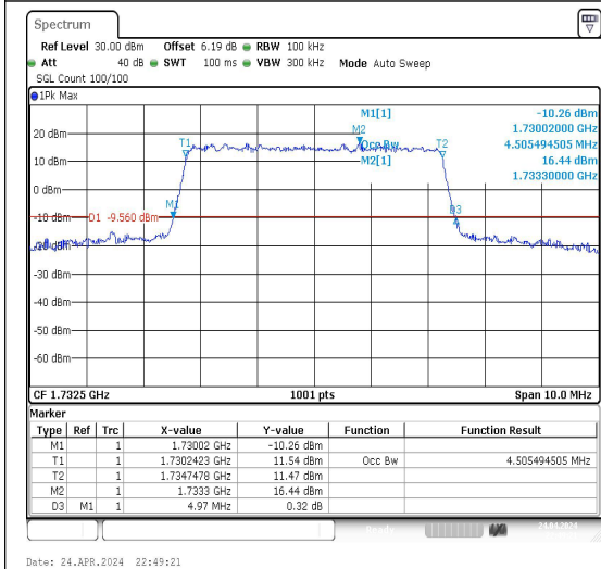
Band4-5MHz-QPSK-20175-25RB#0-PASS
