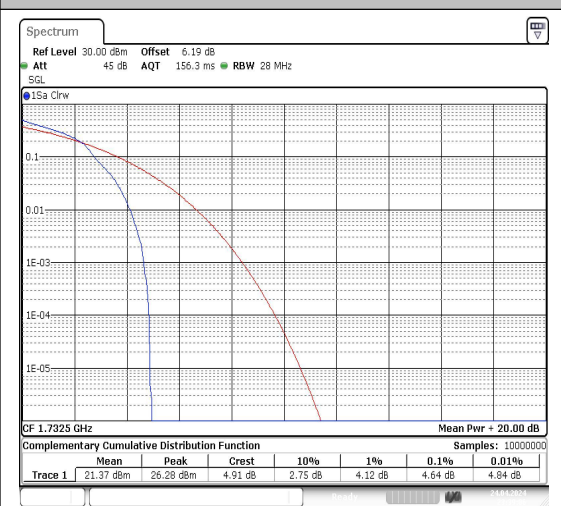
Band4-10MHz-QPSK-20175-1RB#0-PASS
