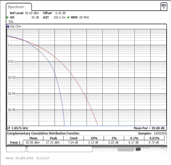
Band2-15MHz-QPSK-18675-75RB#0-PASS Band2-15MHz-16QAM-18675-75RB#0-PASS
