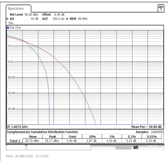
Band2-15MHz-QPSK-18675-1RB#0-PASS Band2-15MHz-16QAM-18675-1RB#0-PASS
