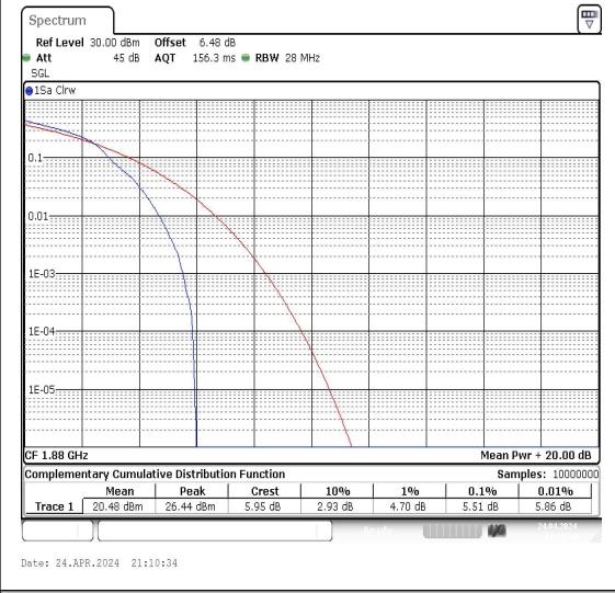
Band2-15MHz-QPSK-18900-1RB#0-PASS Band2-15MHz-16QAM-18900-1RB#0-PASS
