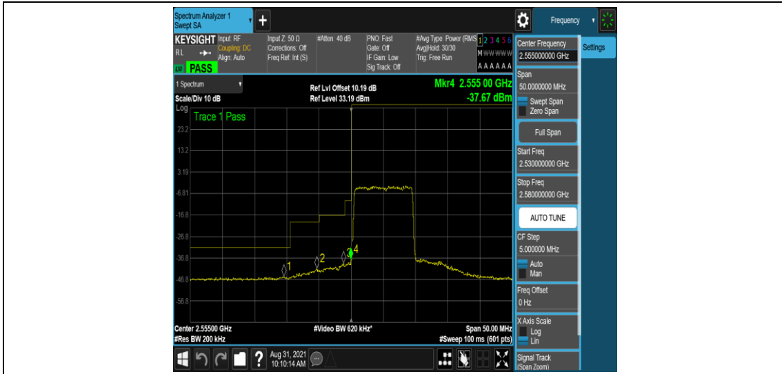
Band41-10MHz-16QAM-40290-50RB#0
