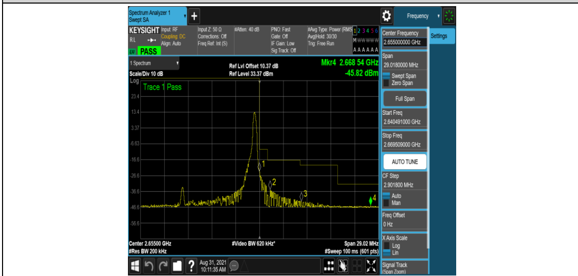
Band41-10MHz-16QAM-41190-1RB#49
