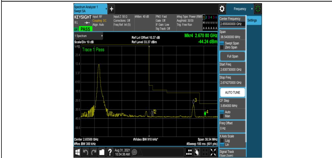
Band41-15MHz-16QAM-41165-1RB#0
