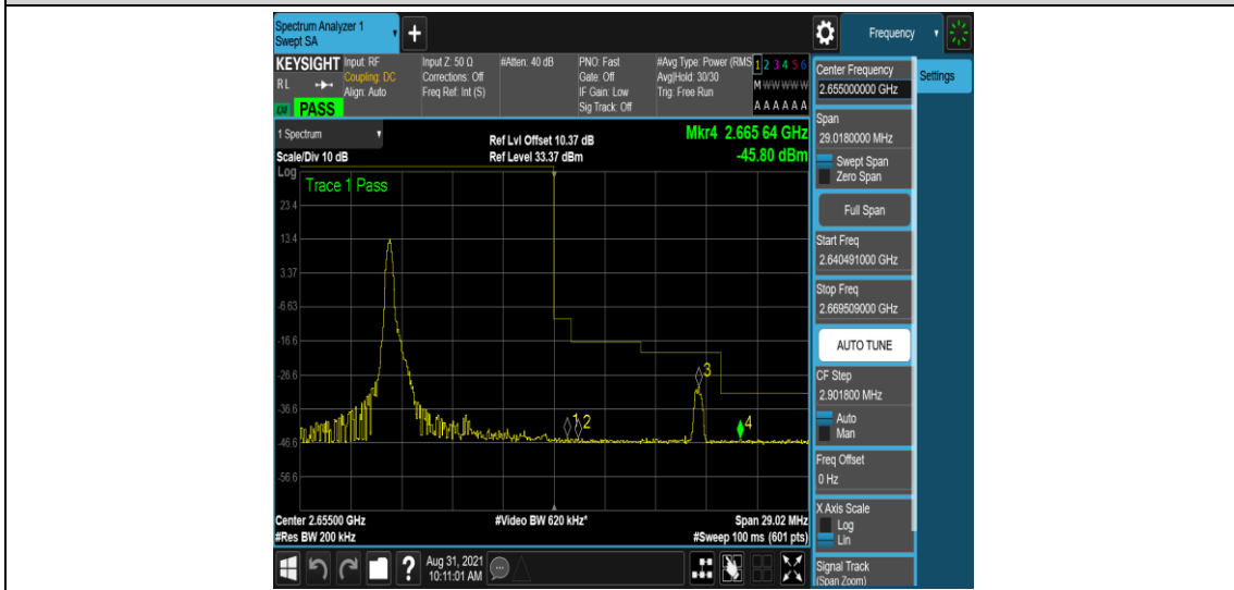
Band41-10MHz-16QAM-41190-1RB#0
