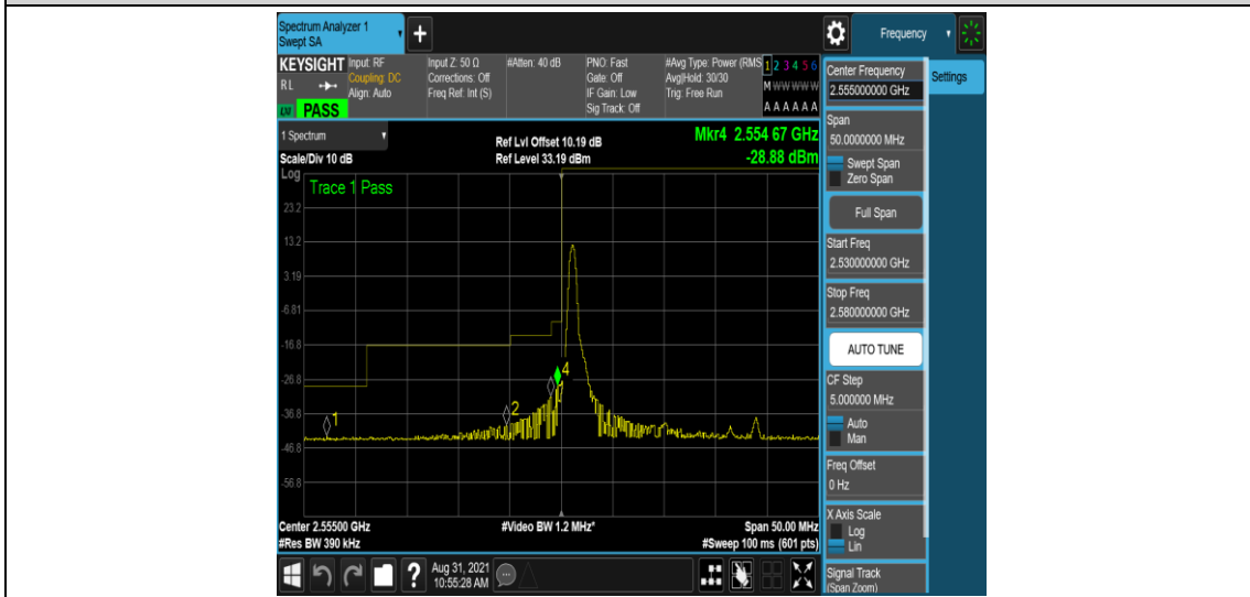
Band41-20MHz-16QAM-40340-1RB#0
