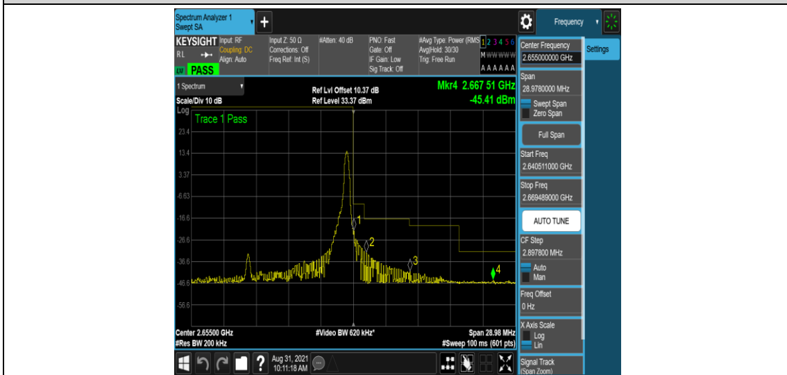
Band41-10MHz-QPSK-41190-1RB#49
