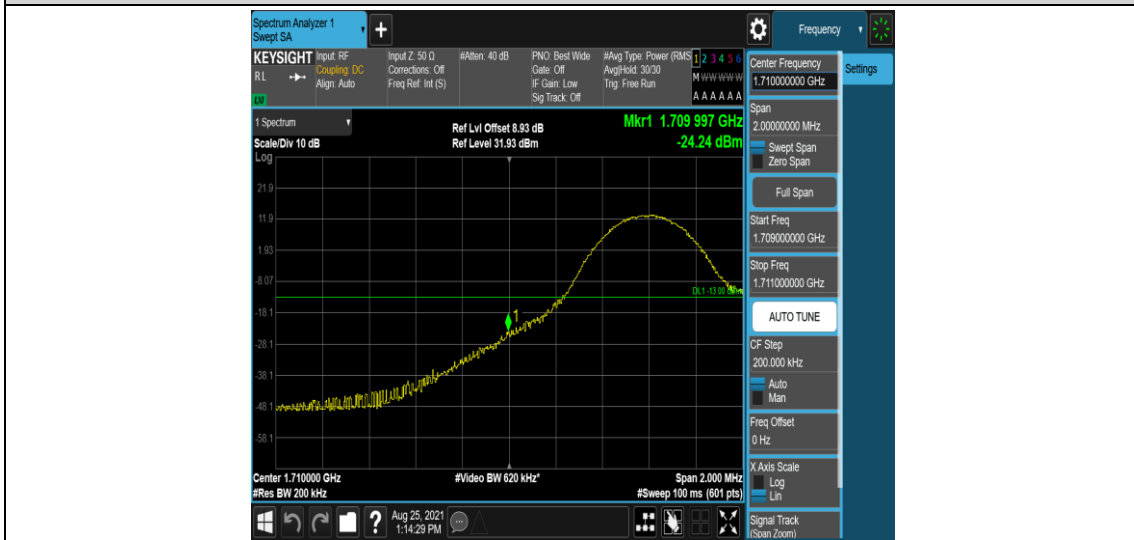
Band4-10MHz-16QAM-20000-1RB#49
