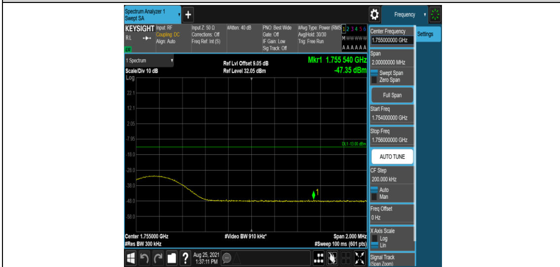
Band4-15MHz-QPSK-20325-1RB#74
