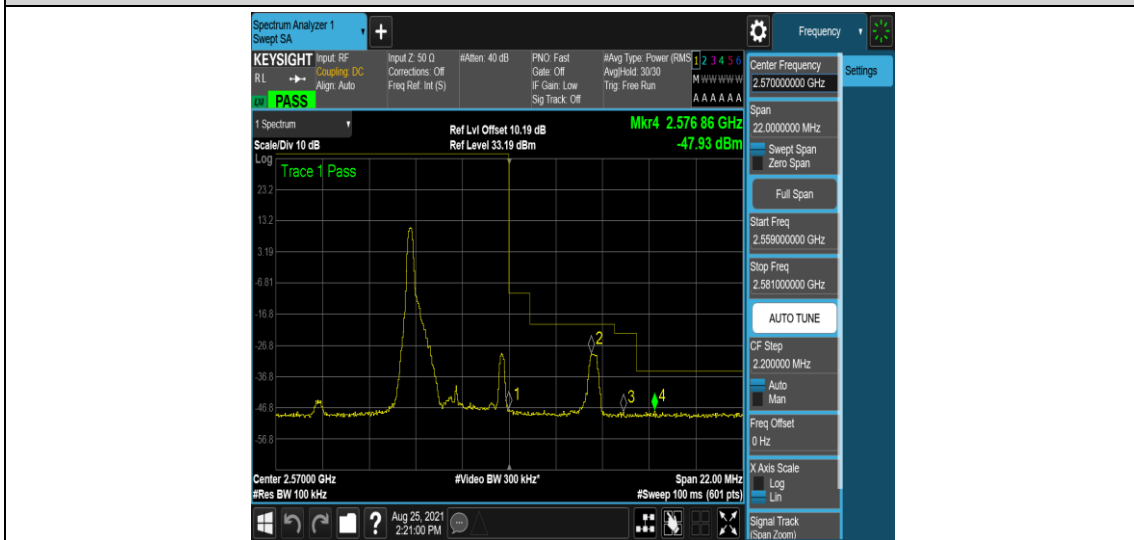
Band7-5MHz-16QAM-21425-1RB#24
