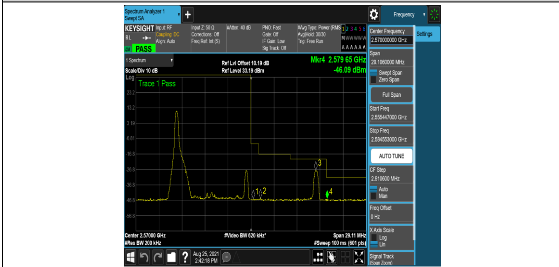
Band7-10MHz-QPSK-21400-1RB#49
