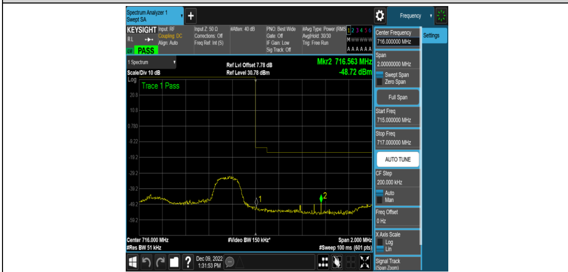
Band12-3MHz-16QAM-23165-1RB#14
