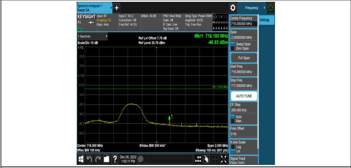
Band12-5MHz-16QAM-23155-1RB#24
