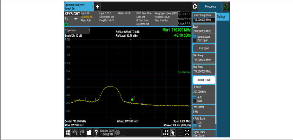
Band12-5MHz-QPSK-23155-1RB#24
