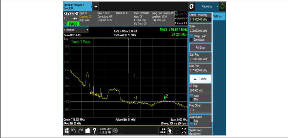
Band12-1.4MHz-QPSK-23173-1RB#5
