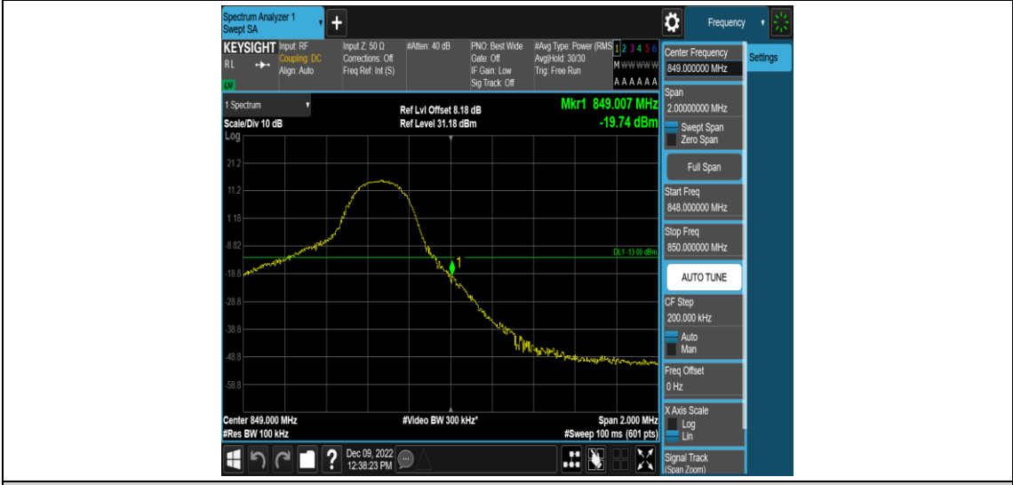
Band5-5MHz-QPSK-20625-25RB#0
