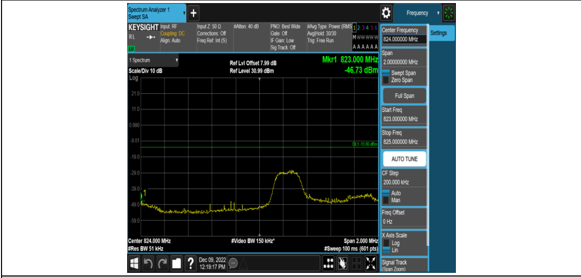
Band5-3MHz-16QAM-20415-15RB#0
