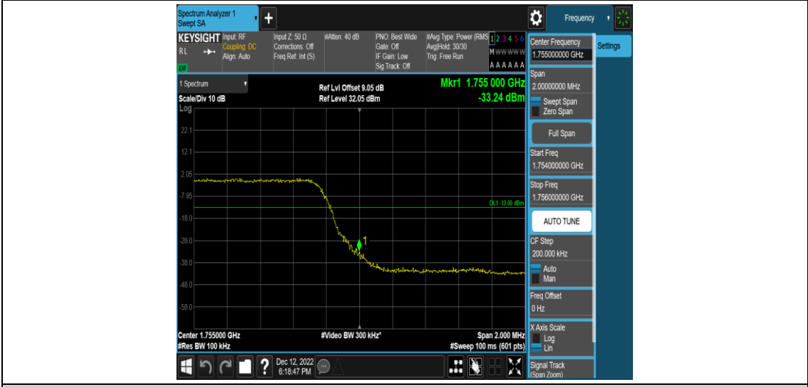
Band4-5MHz-16QAM-19975-1RB#0
