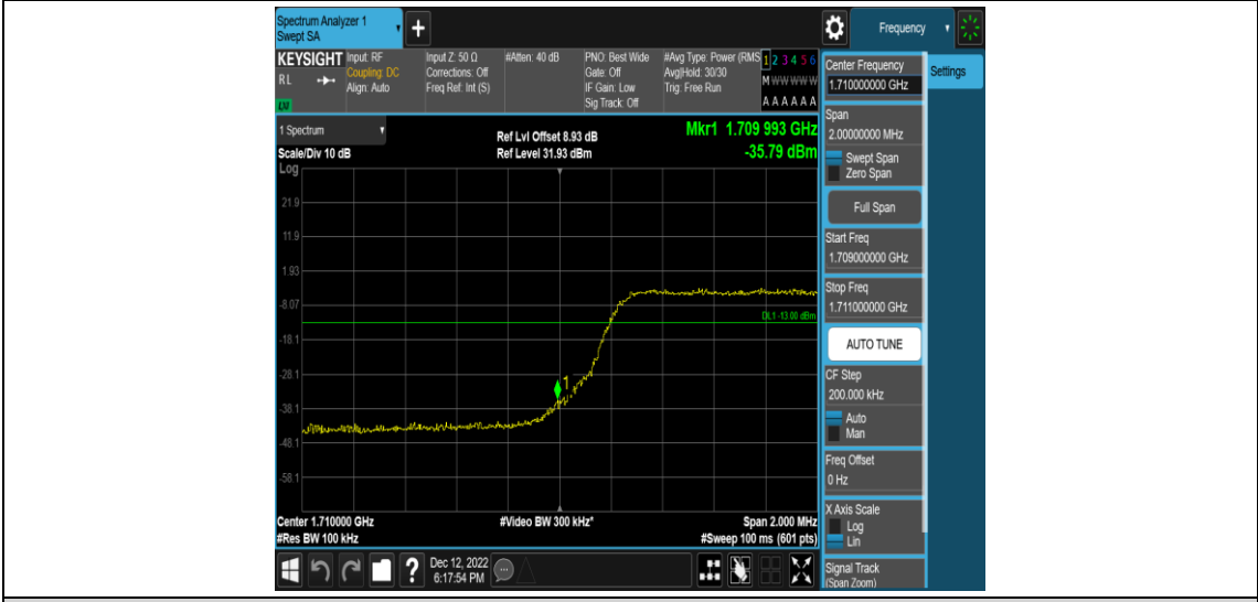
Band4-5MHz-16QAM-20375-1RB#0
