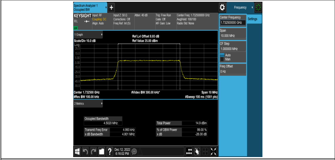
Band4-5MHz-QPSK-20375-25RB#0
