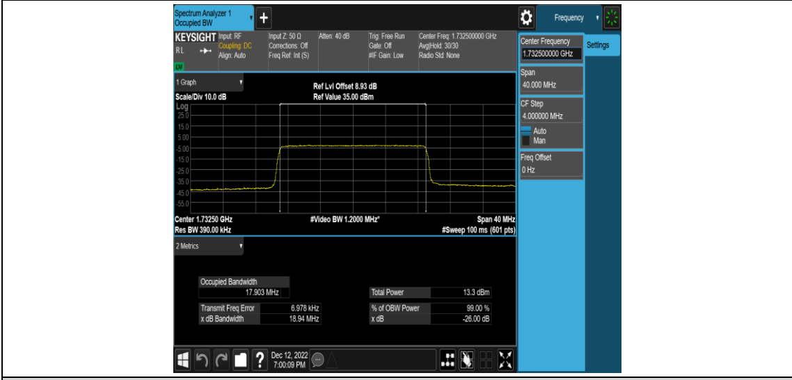
Band4-20MHz-QPSK-20300-100RB#0
