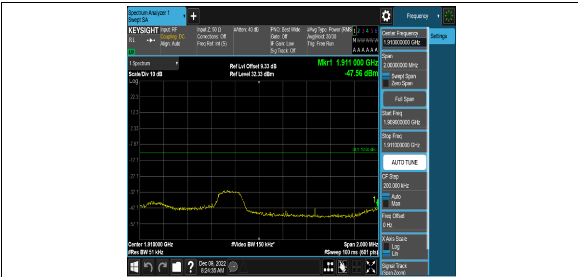
Band2-3MHz-16QAM-19185-1RB#14
