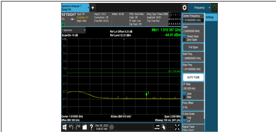
Band2-15MHz-QPSK-19125-1RB#74
