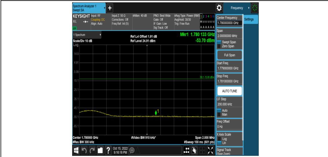
Band66-15MHz-16QAM-132597-1RB#74
