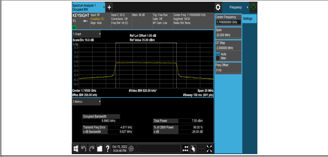
Band66-10MHz-16QAM-132622-50RB#0
