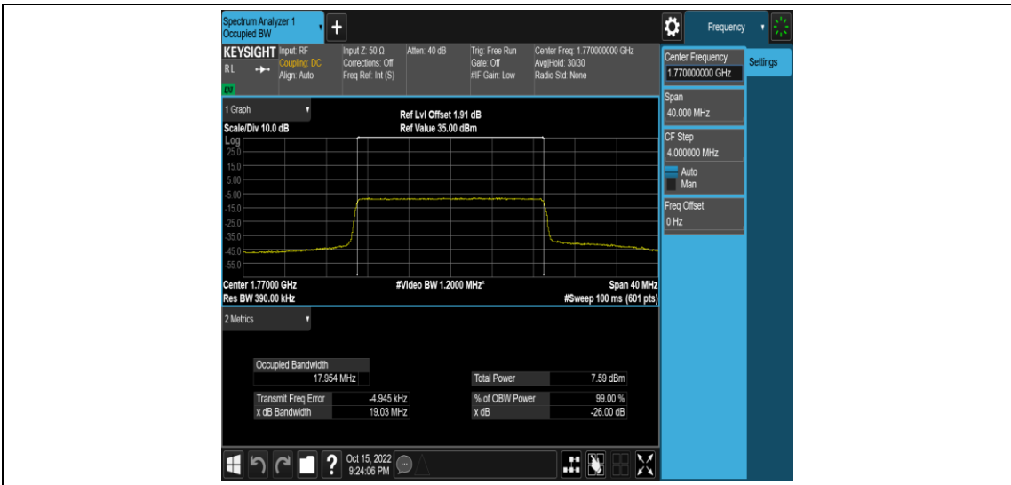
Band66-20MHz-16QAM-132072-100RB#0
