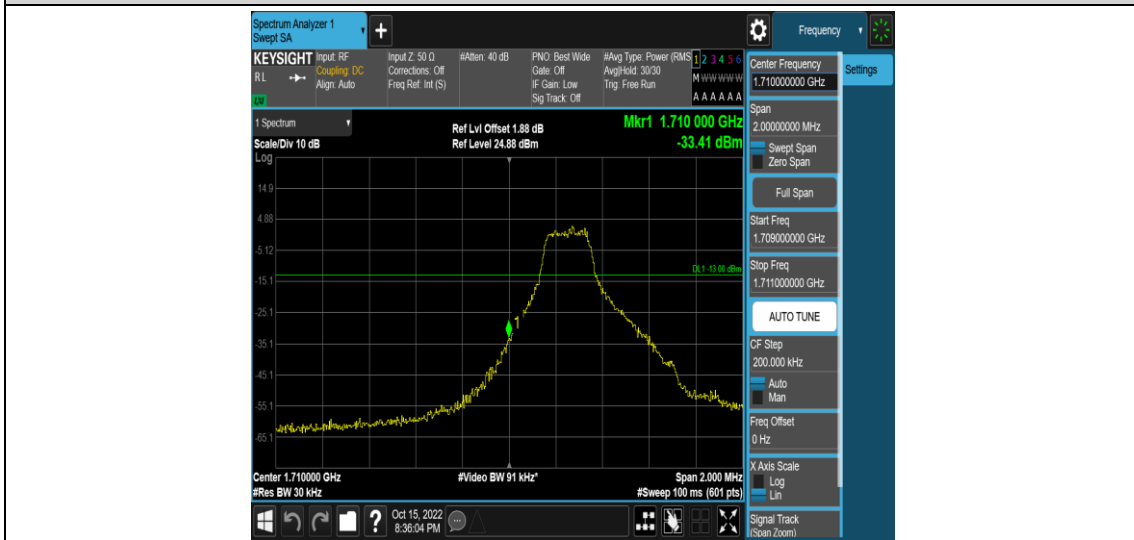
Band66-1.4MHz-16QAM-131979-1RB#5
