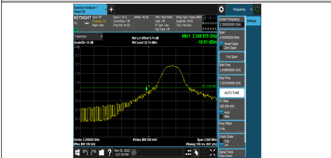
Band40-5MHz-16QAM-39175-1RB#24
