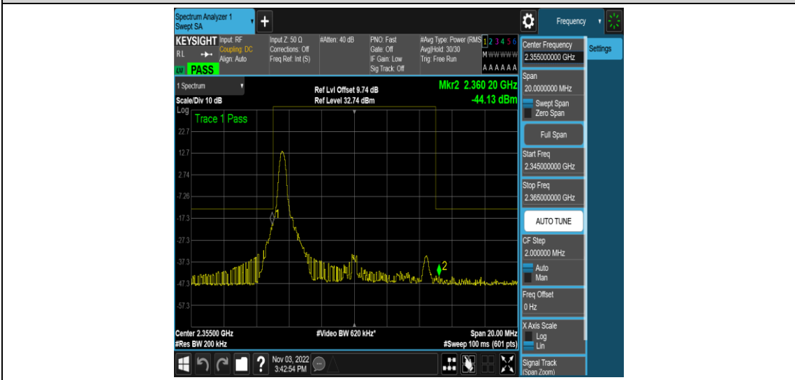
Band40-10MHz-QPSK-39200-1RB#49
