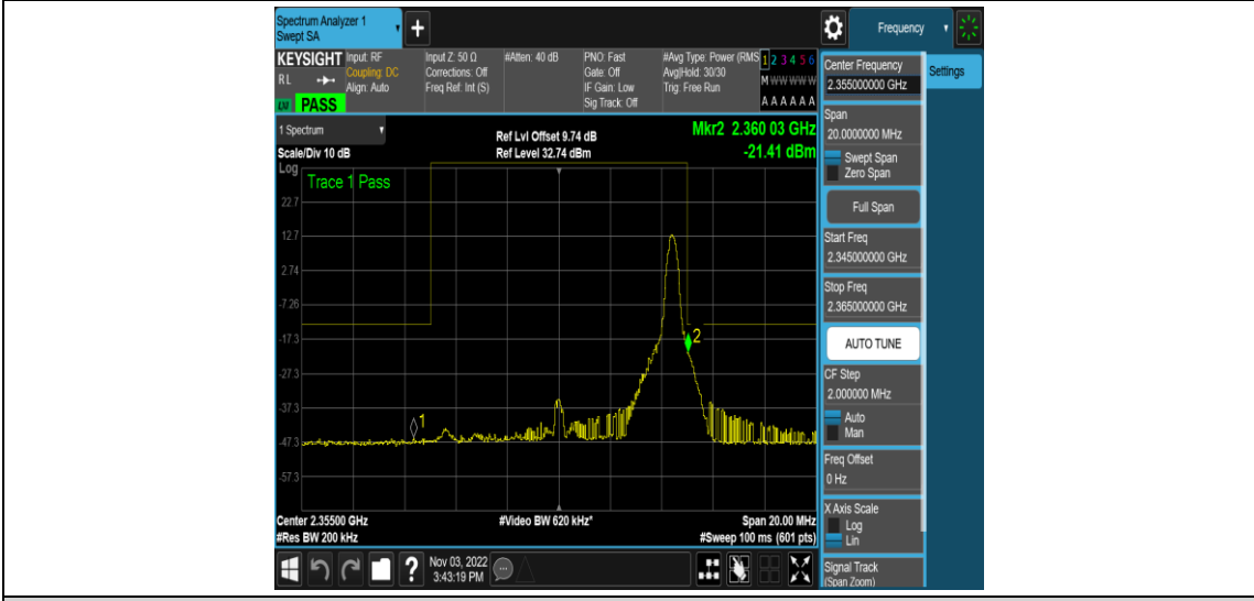
Band40-10MHz-16QAM-39200-50RB#0
