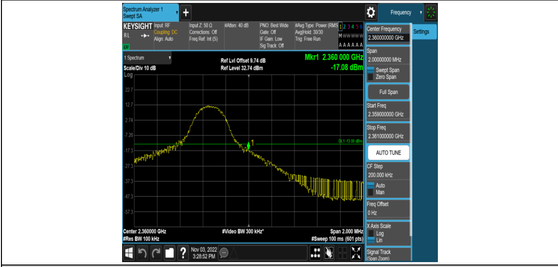
Band40-5MHz-16QAM-39225-25RB#0
