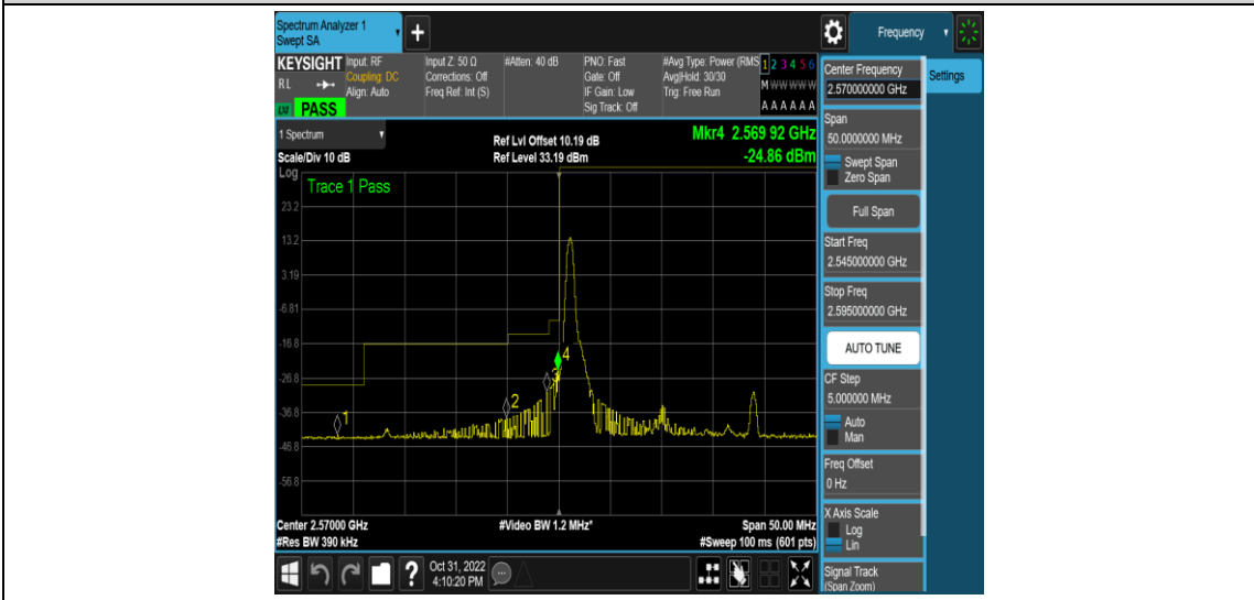
Band38-20MHz-16QAM-37850-1RB#99
