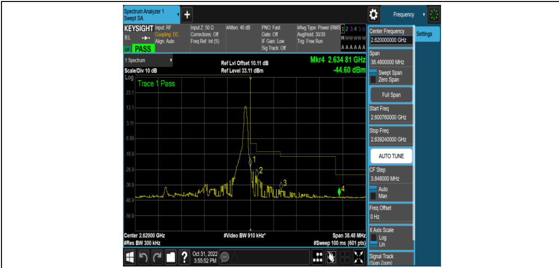
Band38-15MHz-QPSK-38175-75RB#0
