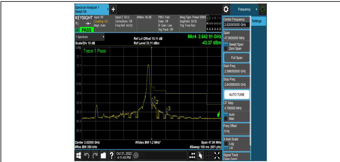
Band38-20MHz-QPSK-38150-100RB#0
