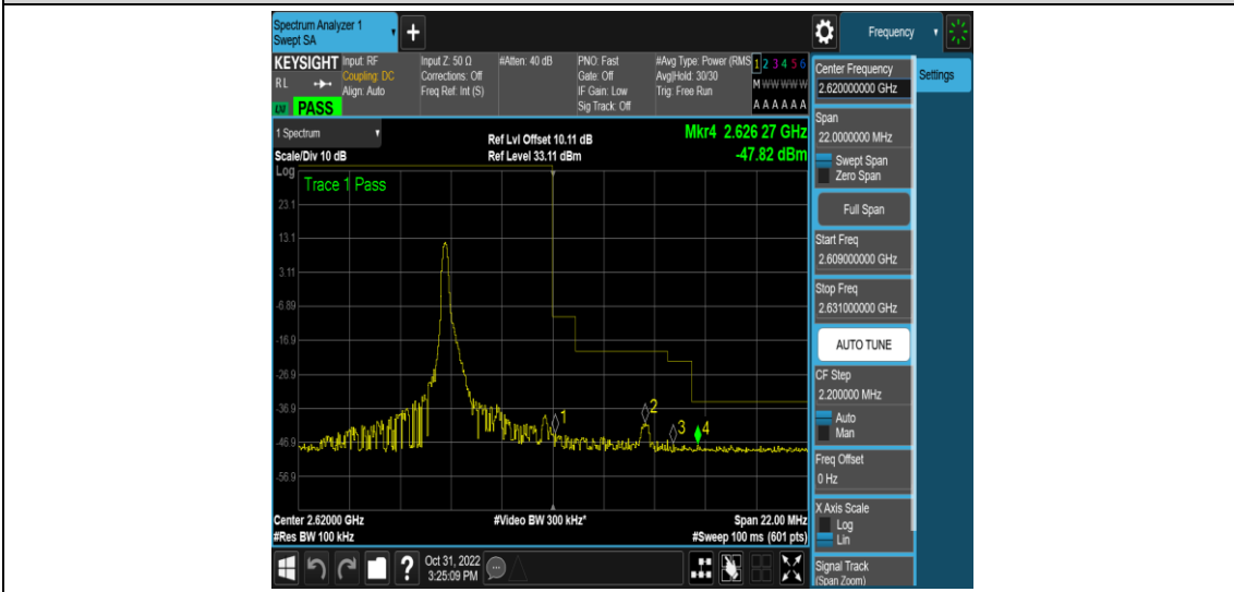
Band38-5MHz-16QAM-38225-1RB#24
