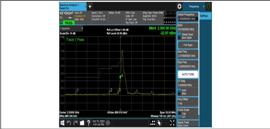
Band7-15MHz-QPSK-20825-1RB#74
