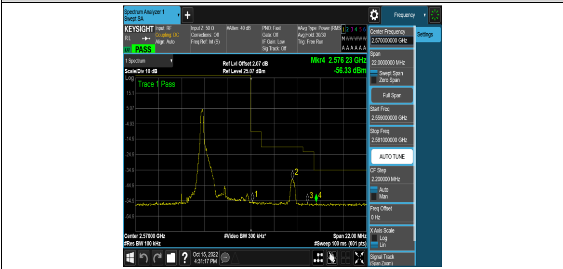
Band7-5MHz-16QAM-21425-1RB#24
