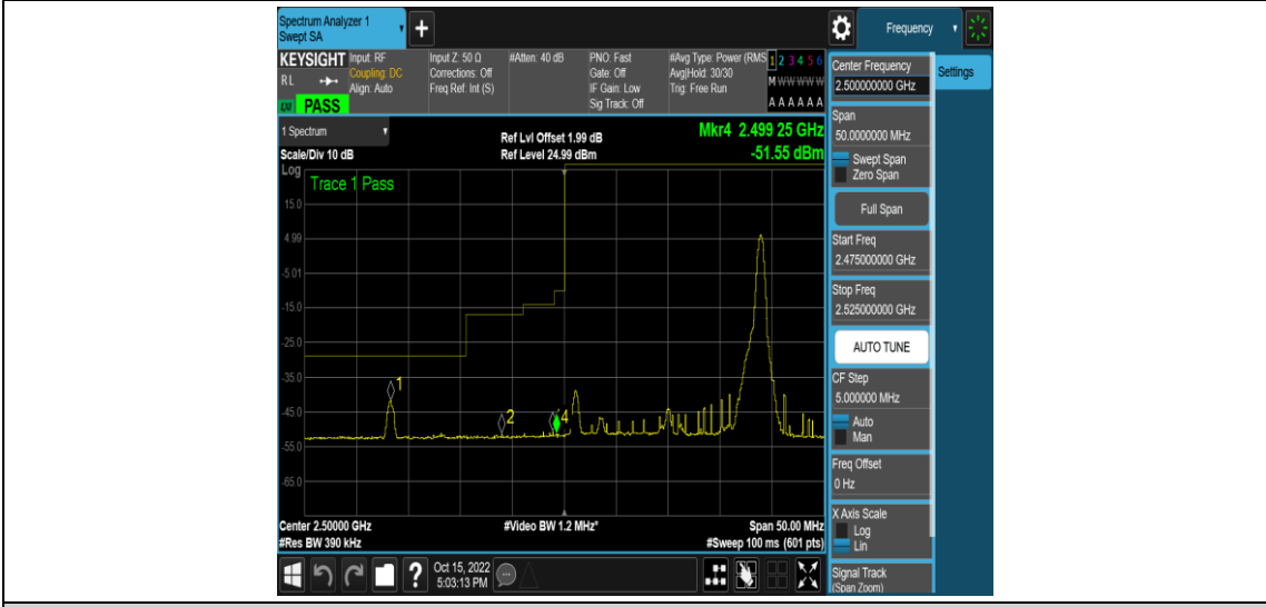
Band7-20MHz-16QAM-20850-100RB#0
