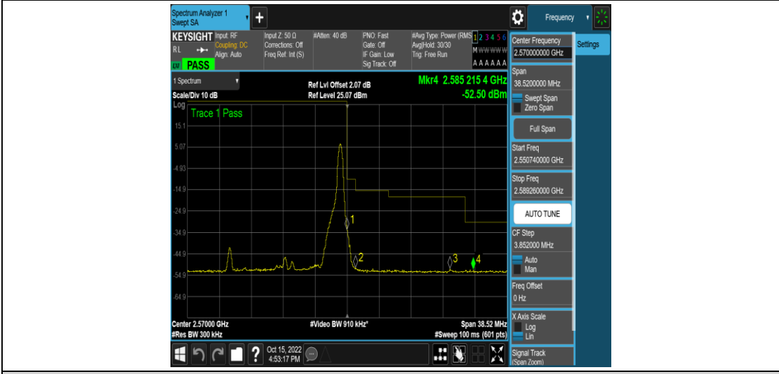
Band7-15MHz-QPSK-21375-75RB#0
