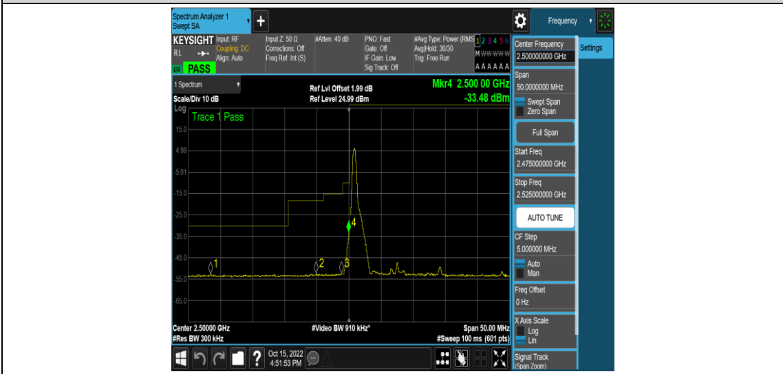
Band7-15MHz-16QAM-20825-1RB#74
