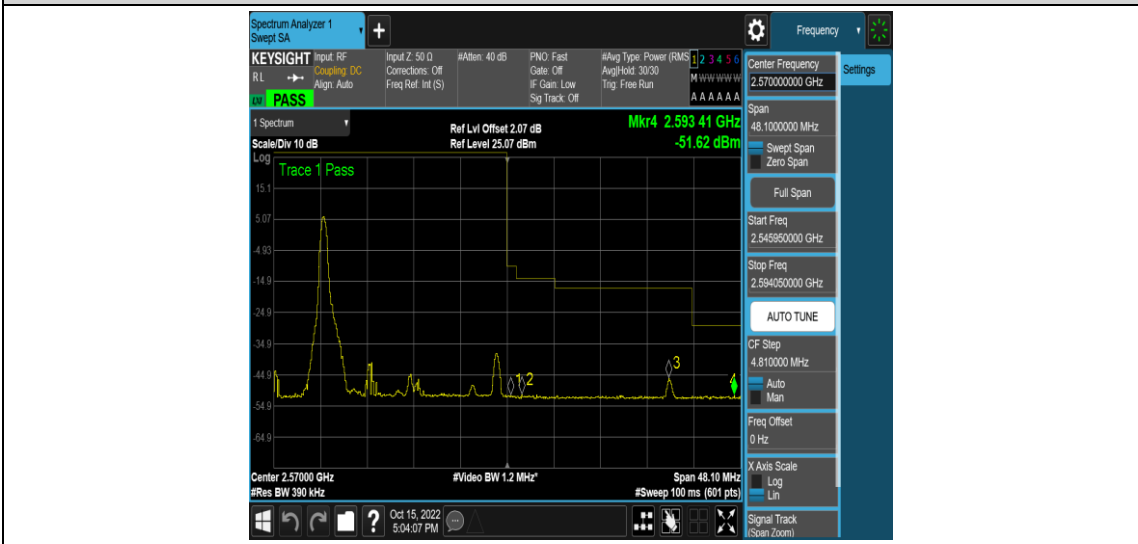
Band7-20MHz-16QAM-21350-1RB#99
