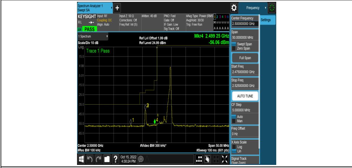
Band7-5MHz-16QAM-20775-25RB#0
