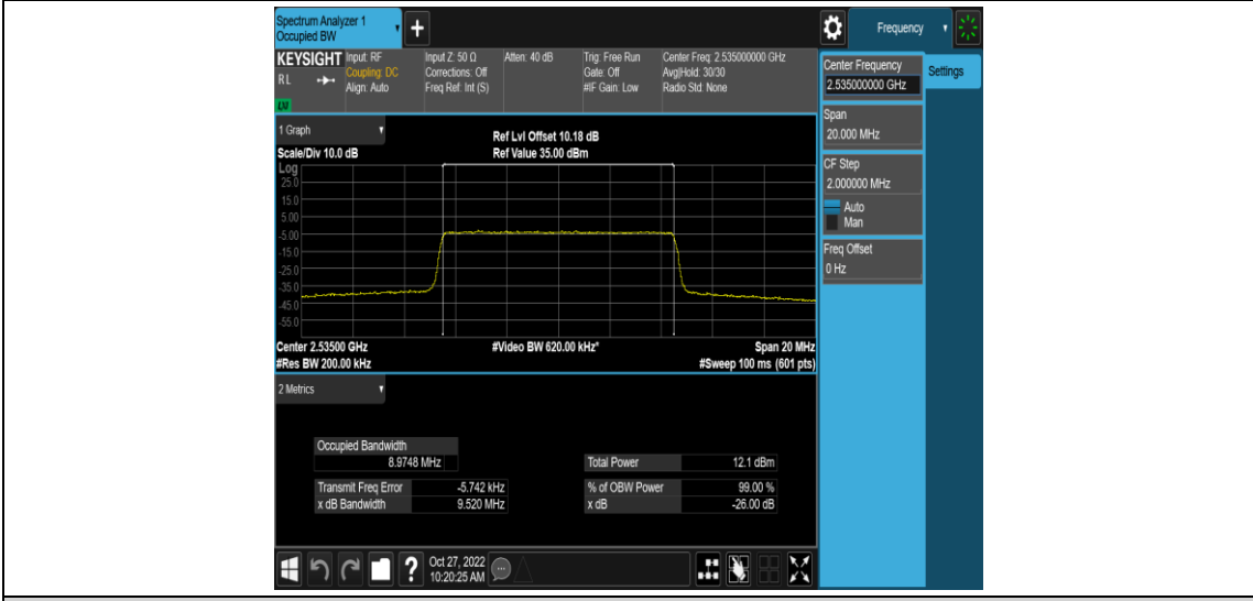
Band7-10MHz-16QAM-21400-50RB#0
