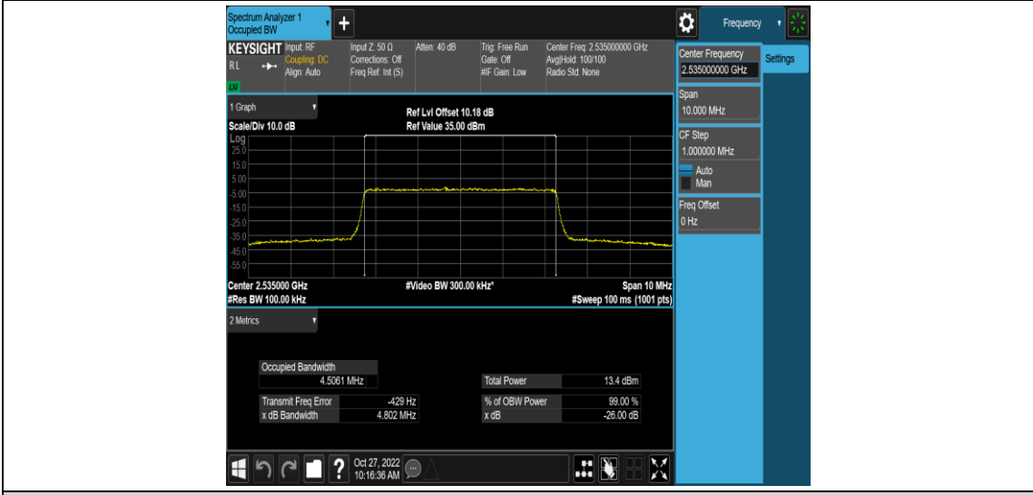
Band7-5MHz-16QAM-21425-25RB#0
