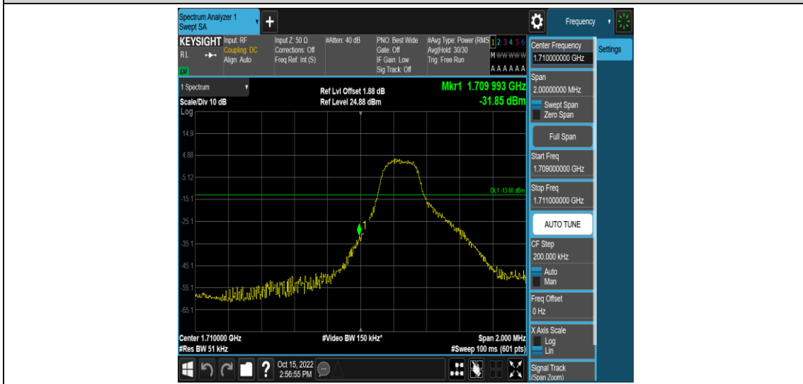
Band4-3MHz-16QAM-19965-1RB#14
