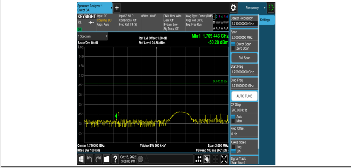
Band4-5MHz-QPSK-19975-25RB#0
