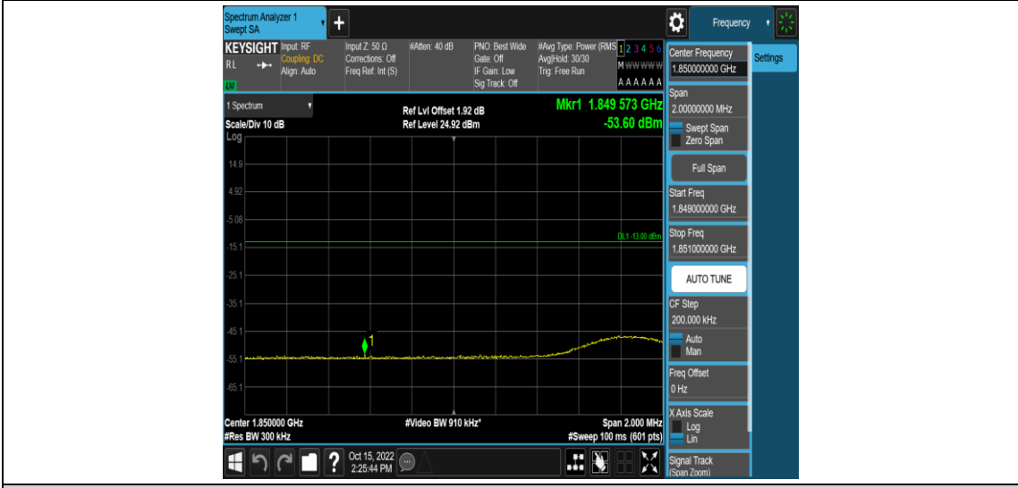
Band2-15MHz-16QAM-18675-75RB#0
