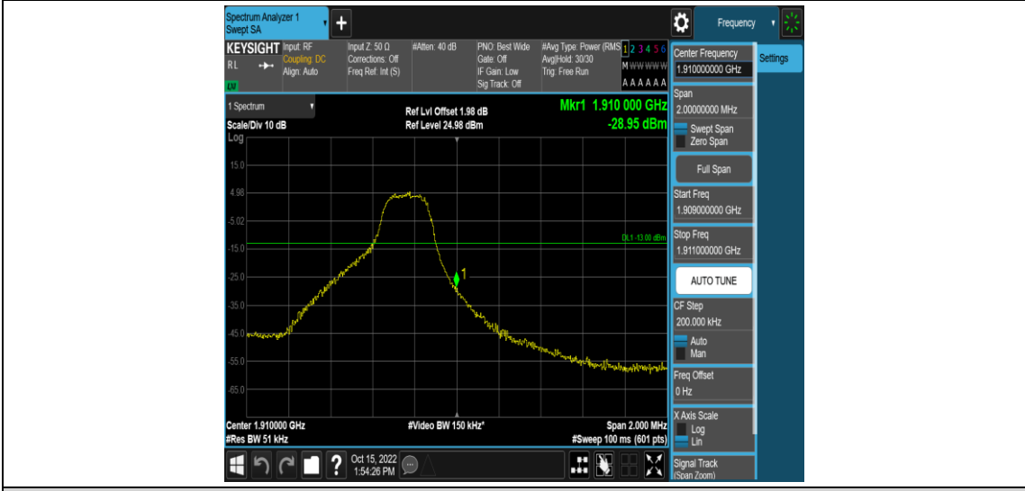
Band2-3MHz-16QAM-19185-15RB#0
