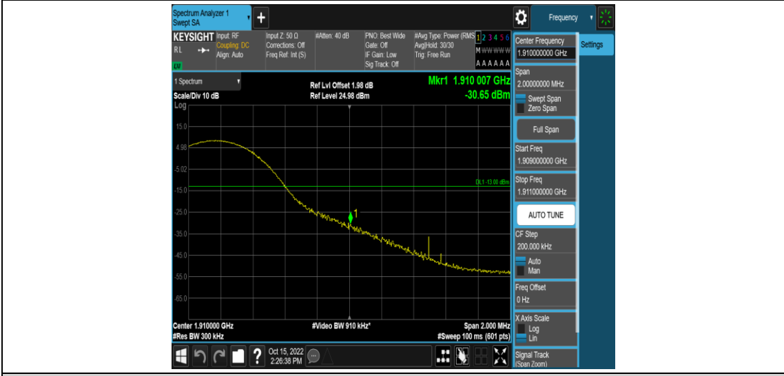
Band2-15MHz-QPSK-19125-75RB#0
