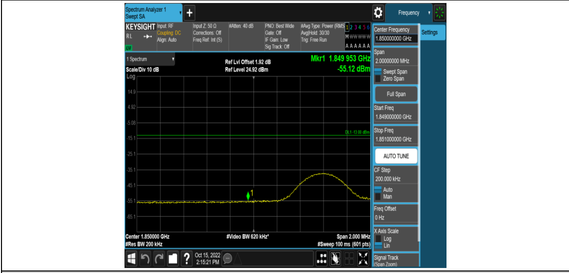
Band2-10MHz-16QAM-18650-50RB#0
