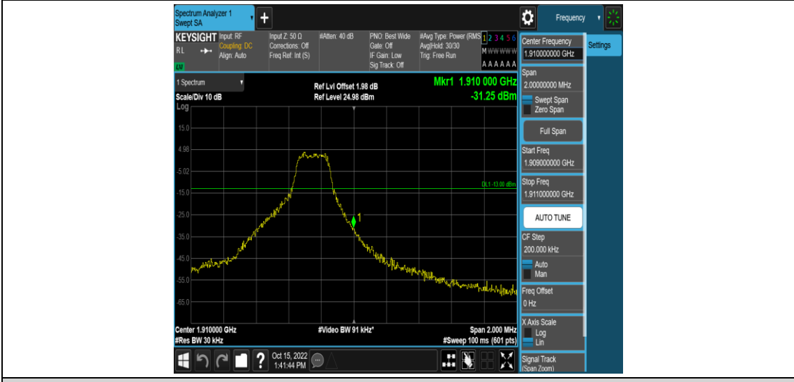
Band2-1.4MHz-16QAM-19193-6RB#0
