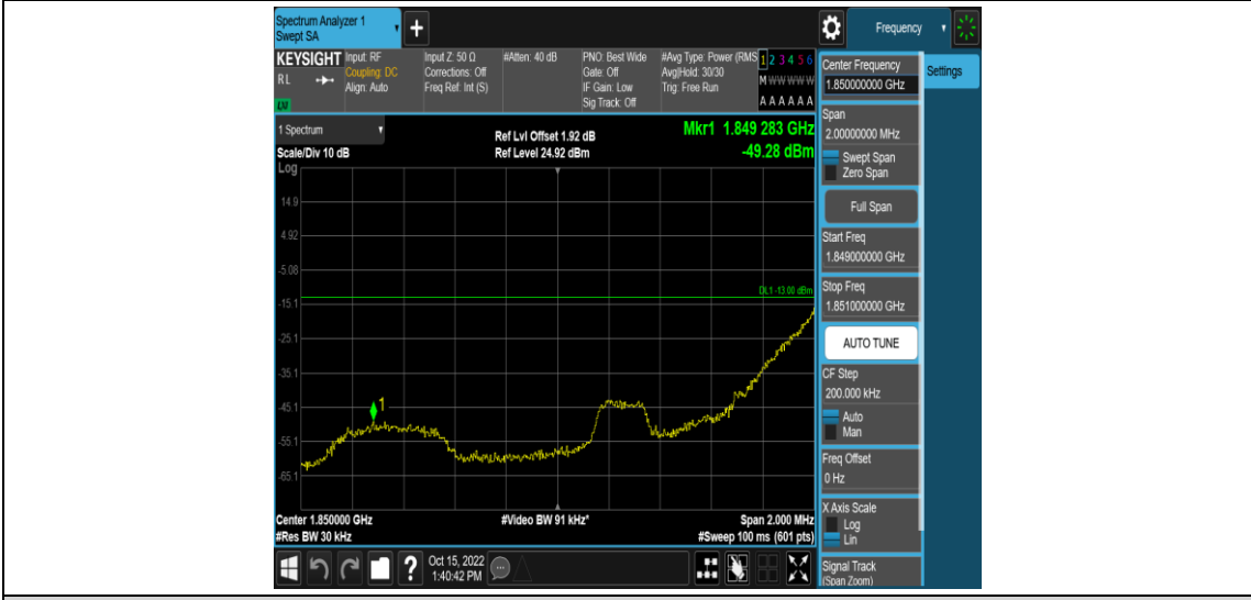
Band2-1.4MHz-16QAM-18607-6RB#0
