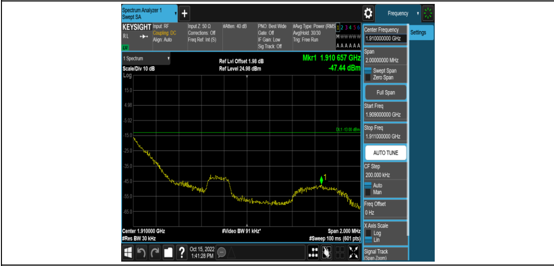
Band2-1.4MHz-16QAM-19193-1RB#5
