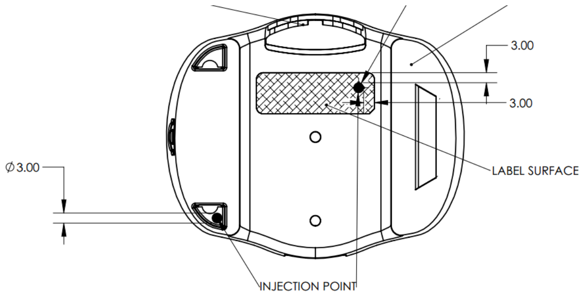
Figure 2: Plastic casing, bottom view, front of device is facing upwards.
