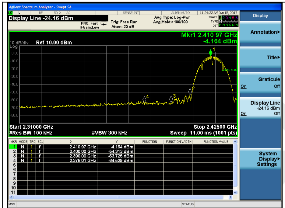
Test Mode: 802.11b---Low
