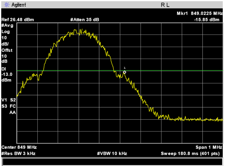
High Band Edge GSM 850 BAND CH 251
