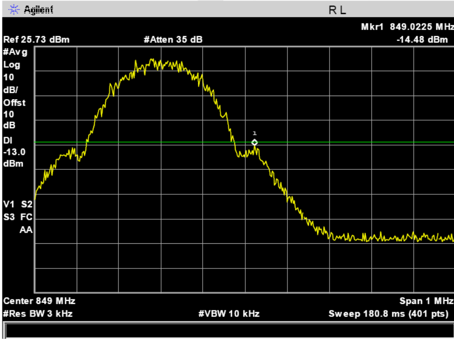
High Band Edge EGPRS 850 BAND CH 251
