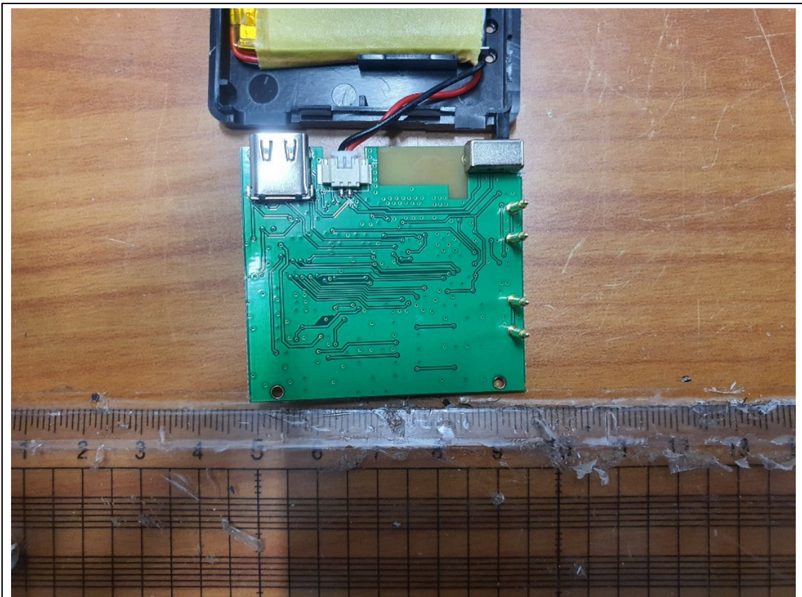
MainBoard-Rear
