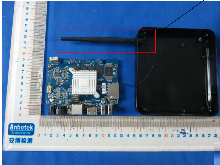
The EUT-Antenna View
