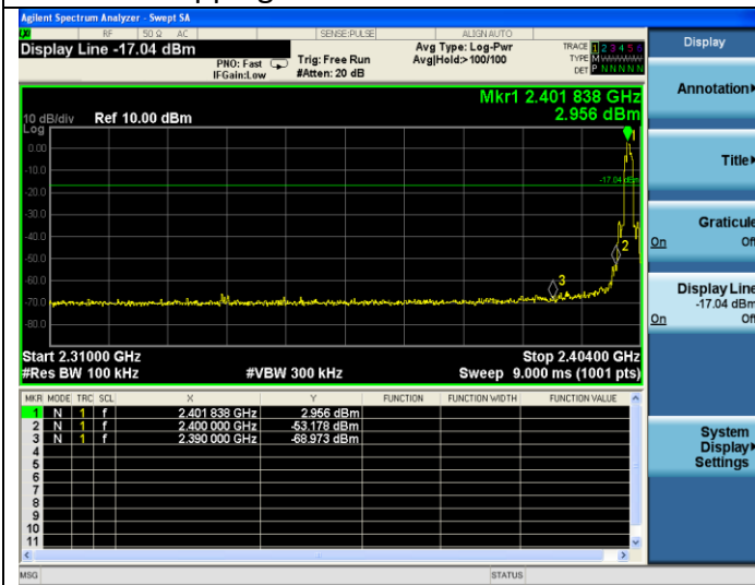
Hopping Off-8-DPSK-Low channel
