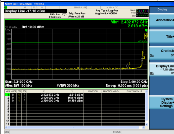
Hopping On-8-DPSK-Low channel
