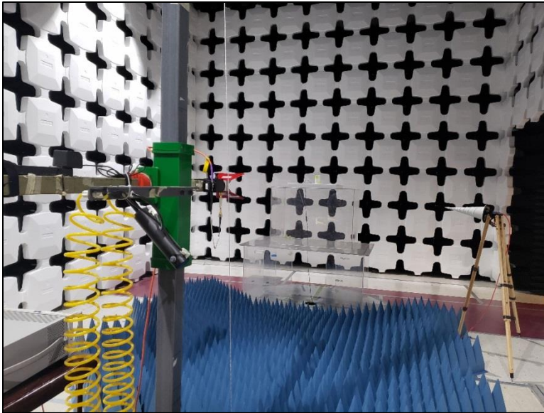
Photograph 2. EIRP, Test Setup, Above 1 GHz
