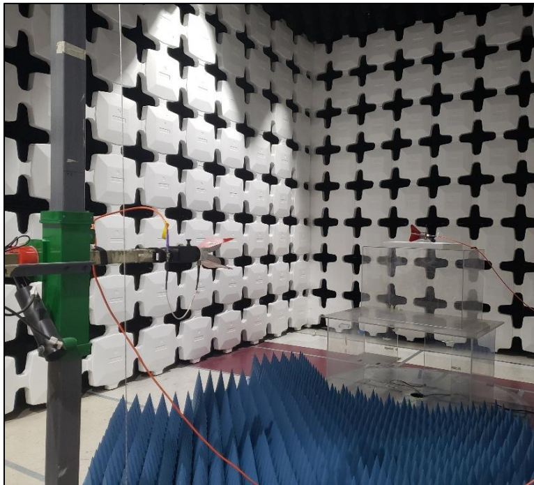
Photograph 4. Radiated Spurious Emissions, Substitution Method, Test Setup
