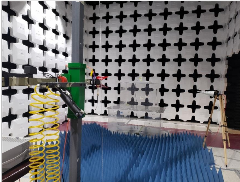
Photograph 3. Radiated Spurious Emissions, Test Setup
