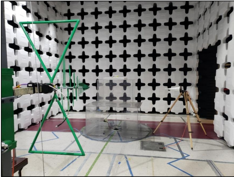
Photograph 1. ERP, Test Setup, Below 1 GHz
