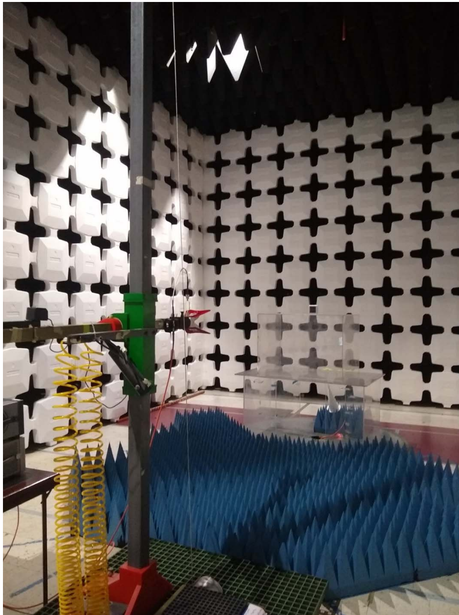
Radiated Spurious Emissions, 1GHz – 18GHz, Test Setup
