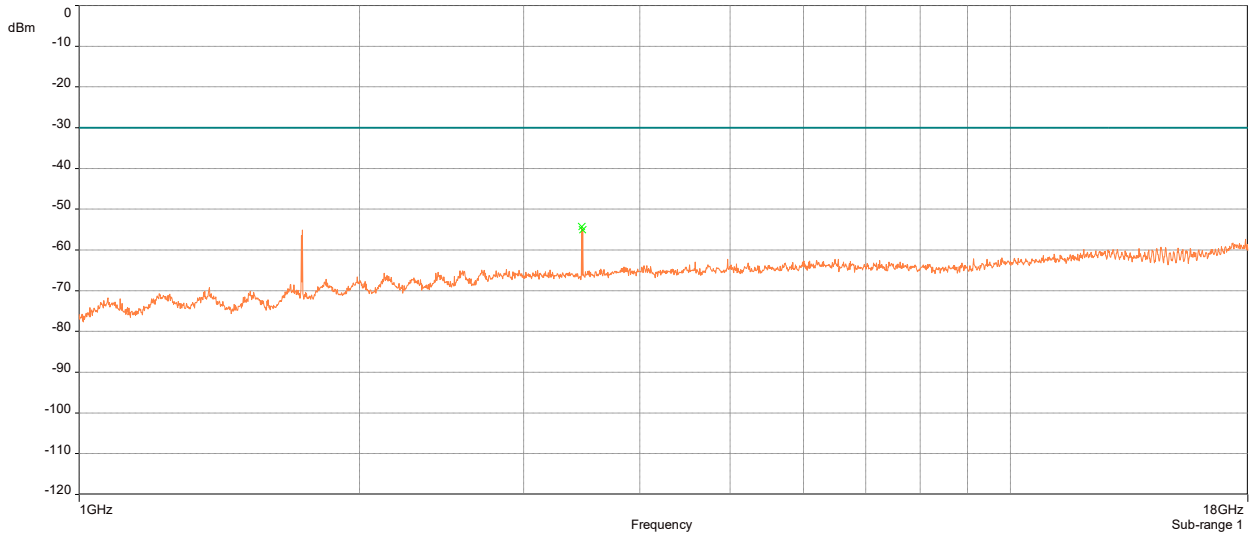
LTE Band 4
