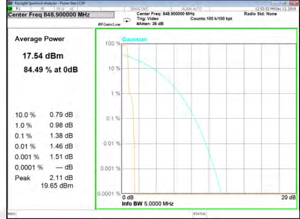
Band5_3.75k_1#0_BPSk_Higher
