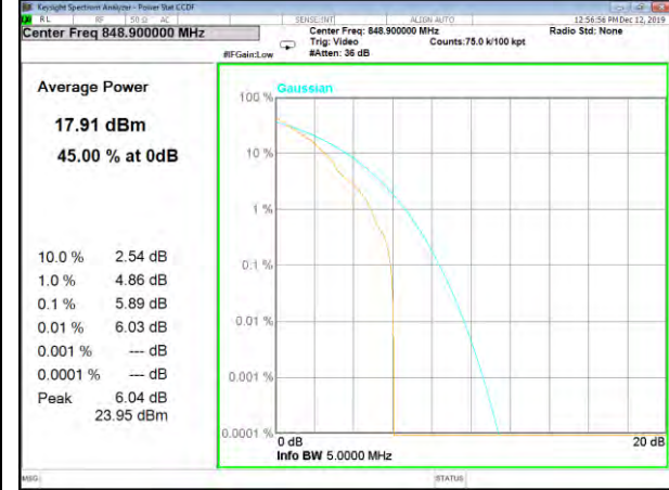
Band5_3.75k_1#0_QPSk_Higher
