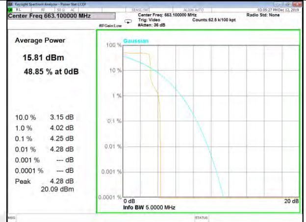
Band71_3.75k_1#0_BPSk_Lower
