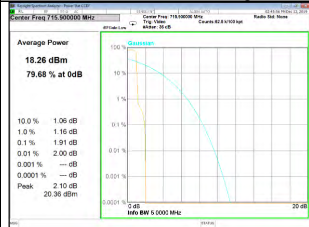
Band12_3.75k_1#0_QPSk_Higher
