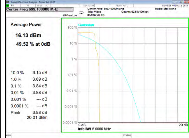
Band12_15k_12#0_QPSk_Lower
