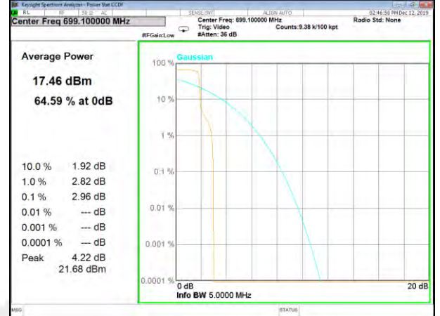
Band12_3.75k_1#0_BPSk_Lower
