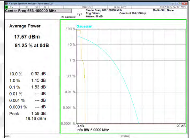
Band71_15k_1#0_BPSk_Middle
