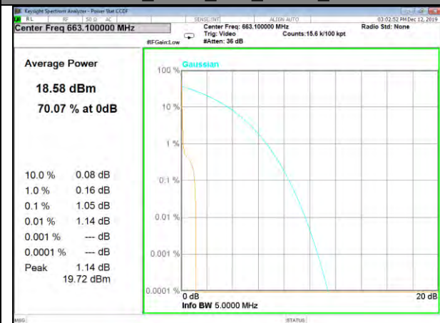
Band71_3.75k_1#0_QPSk_Lower
