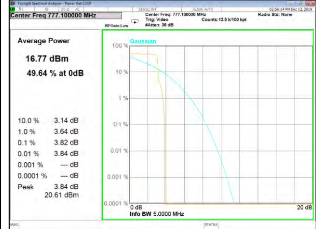
Band13_15k_12#0_QPSk_Lower
