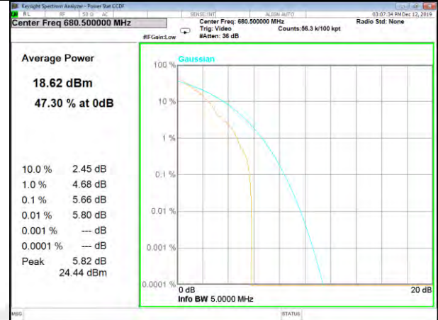
Band71_3.75k_1#0_QPSk_Middle
