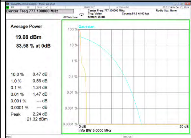
Band13_3.75k_1#0_QPSk_Lower
