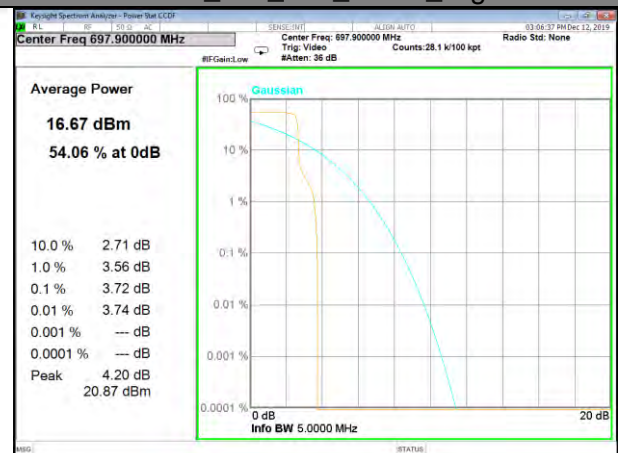
Band71_15k_1#0_QPSk_Higher
