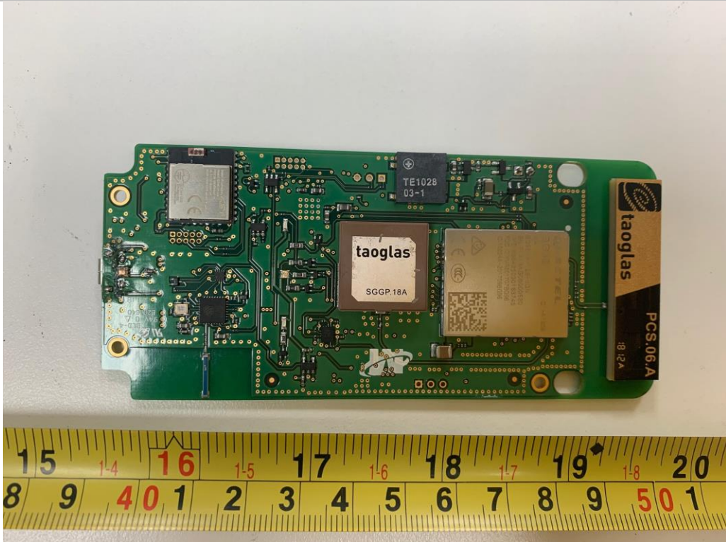
EUT Main PCBA – Top View
