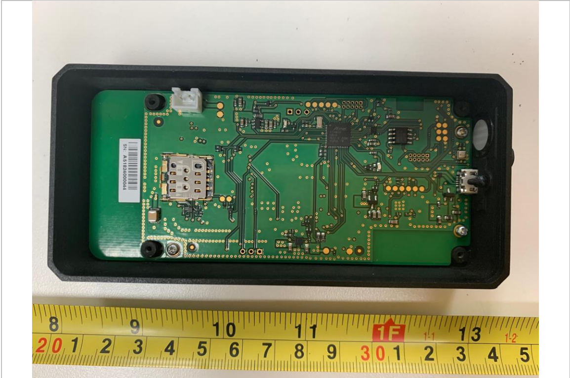
EUT Cover Off View-1
