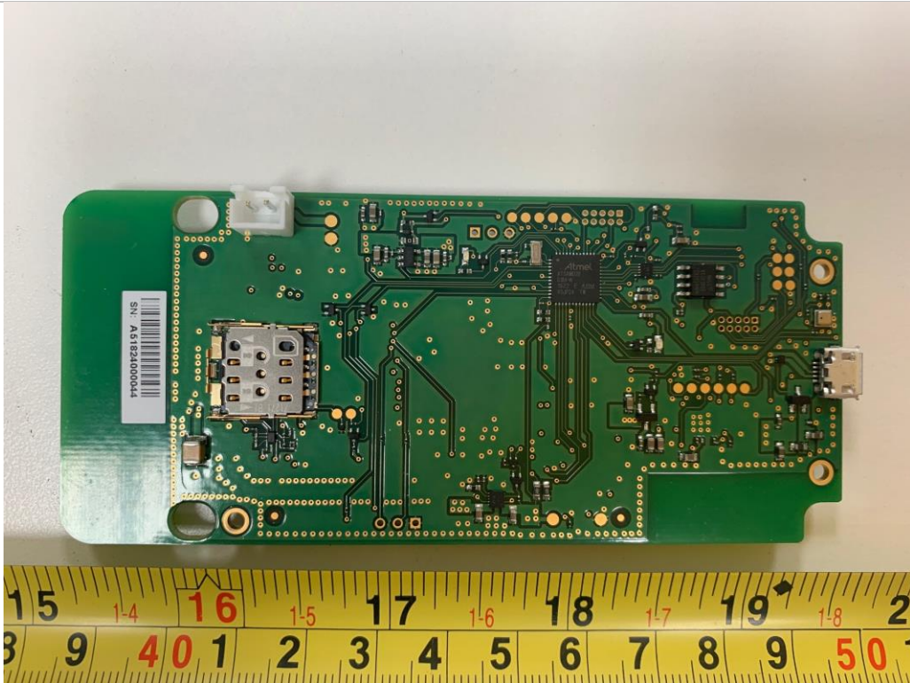
EUT Main PCBA – Bottom View
