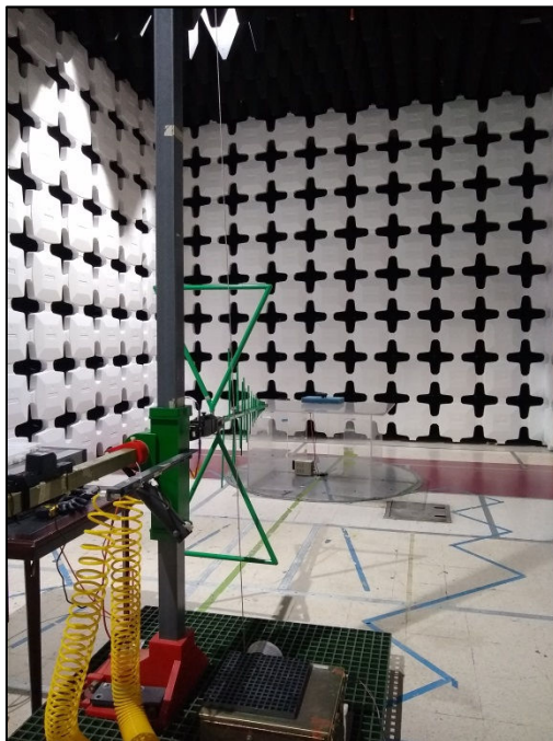
Photograph 3. Radiated Emissions, 30 MHz – 1 GHz, Test Setup
