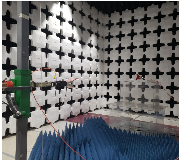
Photograph 5. Radiated Spurious Emissions, Substitution Method Above 1GHz, Test Setup
