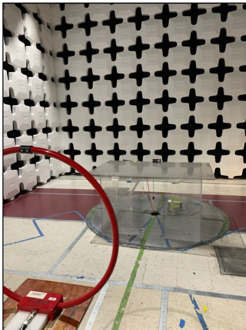
Photograph 1. Radiated Emissions, 10kHz – 30MHz, X-Axis Test Setup
