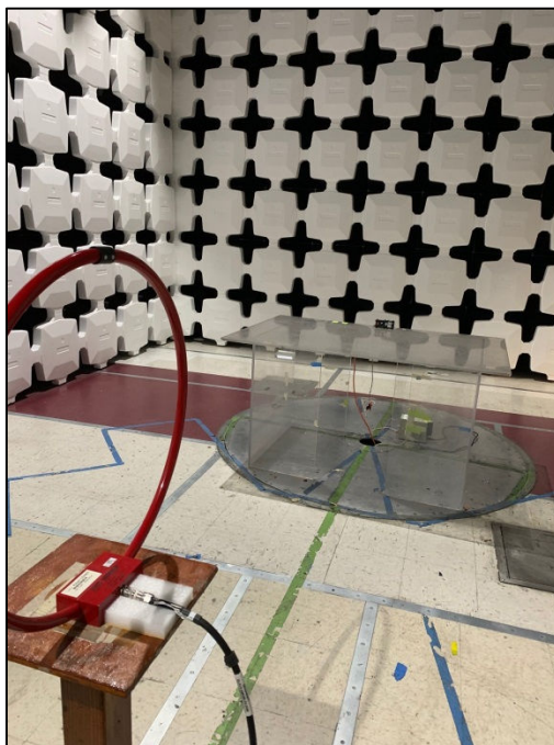
Photograph 2. Radiated Emissions, 10kHz – 30MHz, Y-Axis Test Setup
