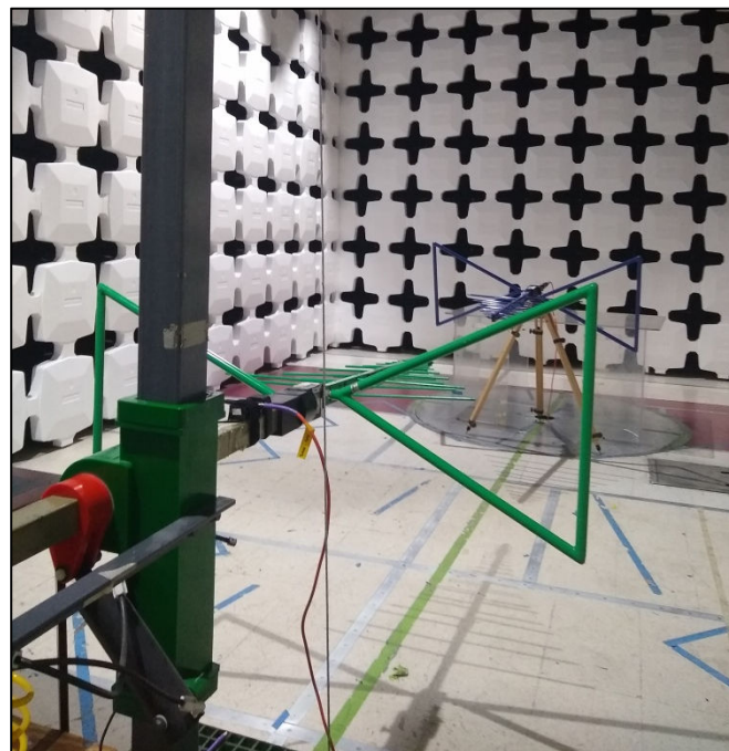
Photograph 6. Radiated Spurious Emissions, Substitution Method Below 1GHz, Test Setup
