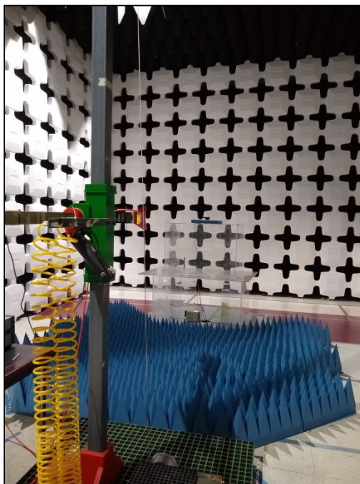
Photograph 4. Radiated Emissions, 1GHz – 18 GHz, Test Setup
