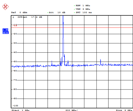
LTE Band 25 5MHz CH-Low 1GHz~3GHz
