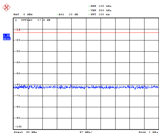
LTE Band 25 5MHz CH-Low 30MHz~1GHz
