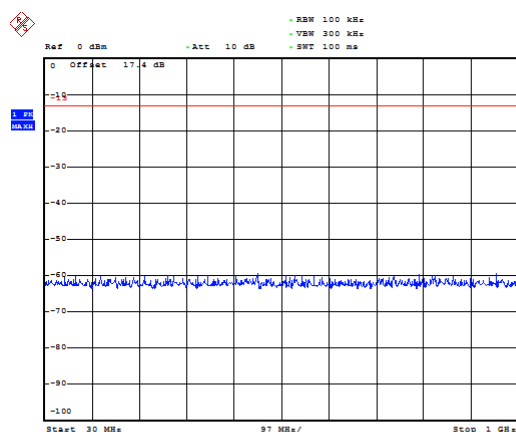
LTE Band 25 5MHz CH-Middle 30MHz~1GHz
