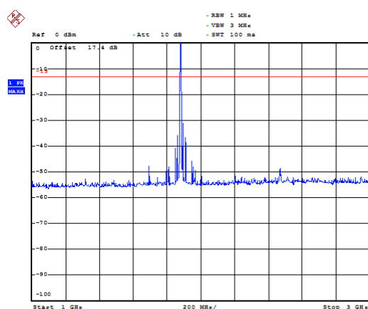
LTE Band 25 5MHz CH-Middle 1GHz~3GHz
