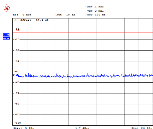
LTE Band 25 5MHz CH-Low 3GHz~20GHz
