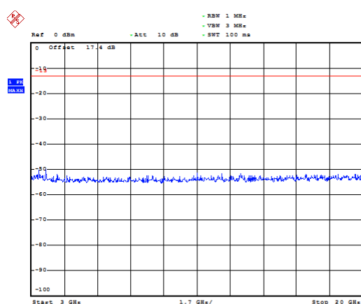
LTE Band 25 5MHz CH-Middle 3GHz~20GHz
