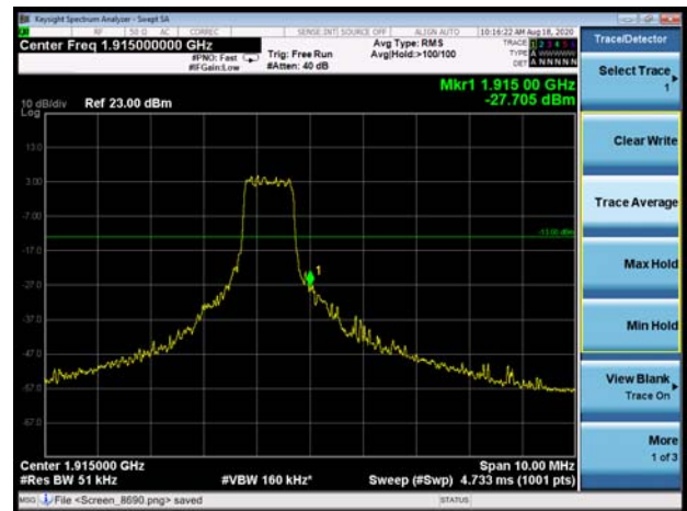
LTE Band 25 5MHz 16QAM 1RB CH-High
