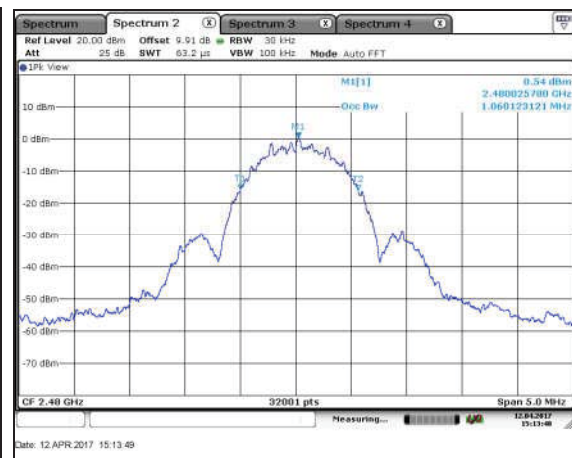
Figure 7.3.2-6: 99% OBW – HCH
