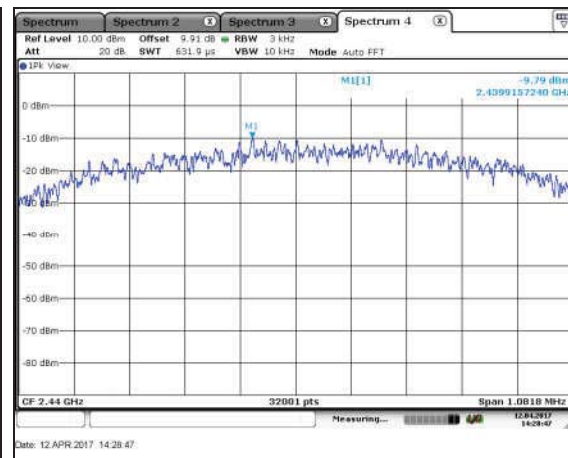
Figure 7.6.2-2: PSD – MCH
