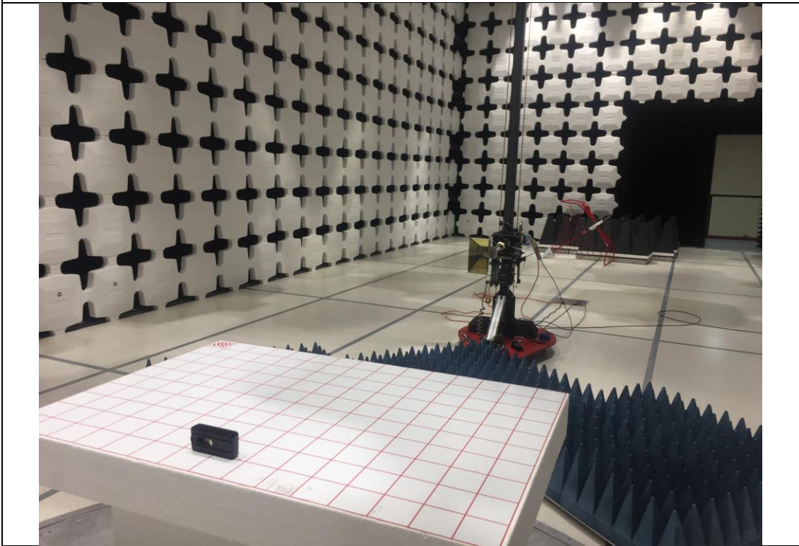
Radiated Emissions Above 1GHz setup for unintentional radiator – Rear
