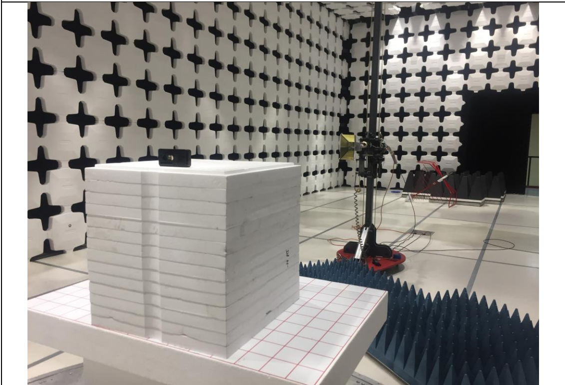
Radiated Emissions Above 1GHz setup for intentional radiator – Rear
