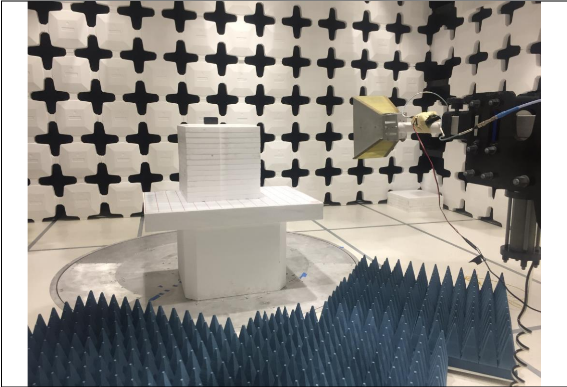
Radiated Emissions Above 1GHz setup for intentional radiator – Front
