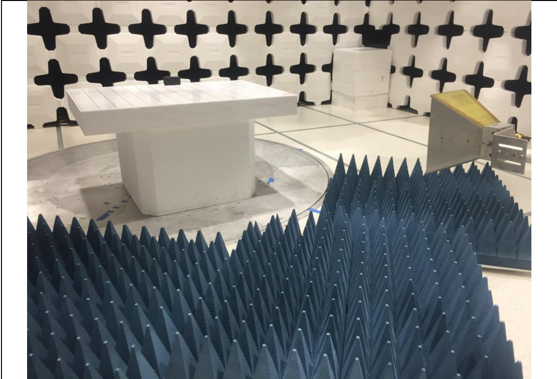
Radiated Emissions Above 1GHz setup for unintentional radiator – Front
