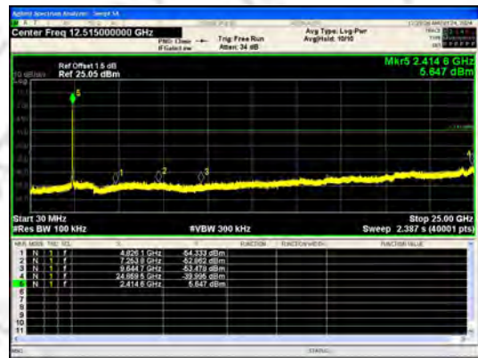
30.0 MHz - 25000.0 MHz IEEE 802.11g_Channel 1_20MHz_Antenna 1
