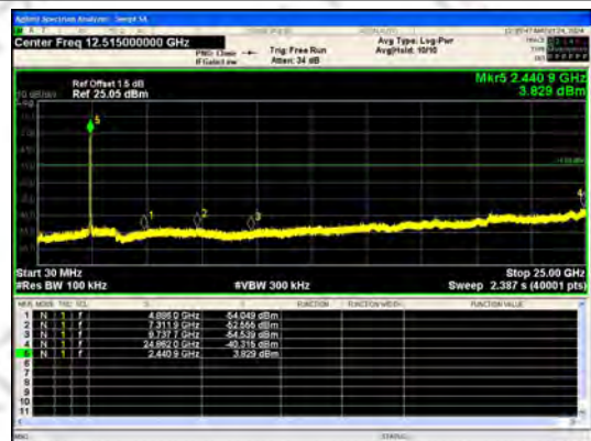
30.0 MHz - 25000.0 MHz IEEE 802.11g_Channel 6_20MHz_Antenna 1
