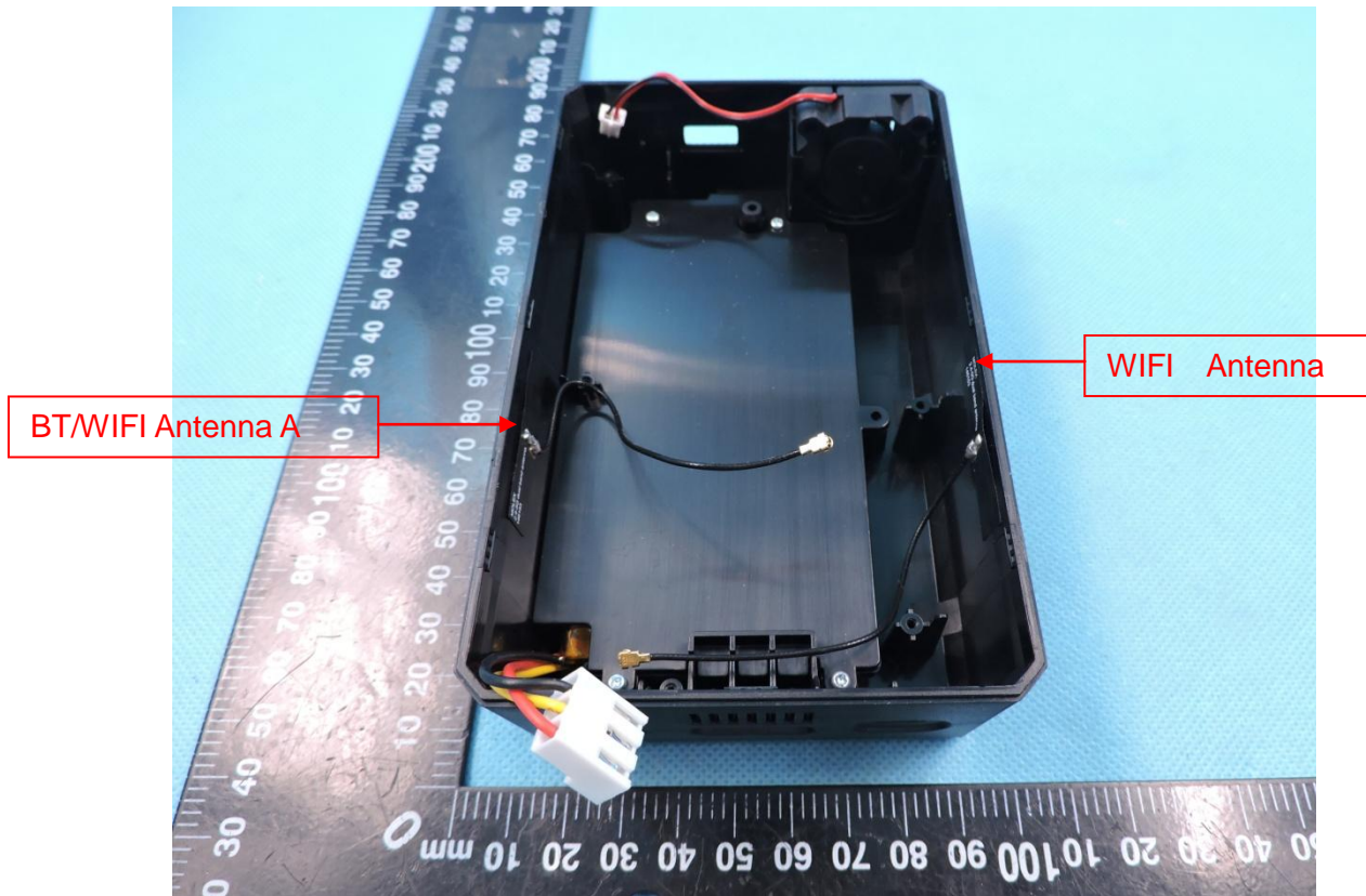
Photo 7_module antenna
